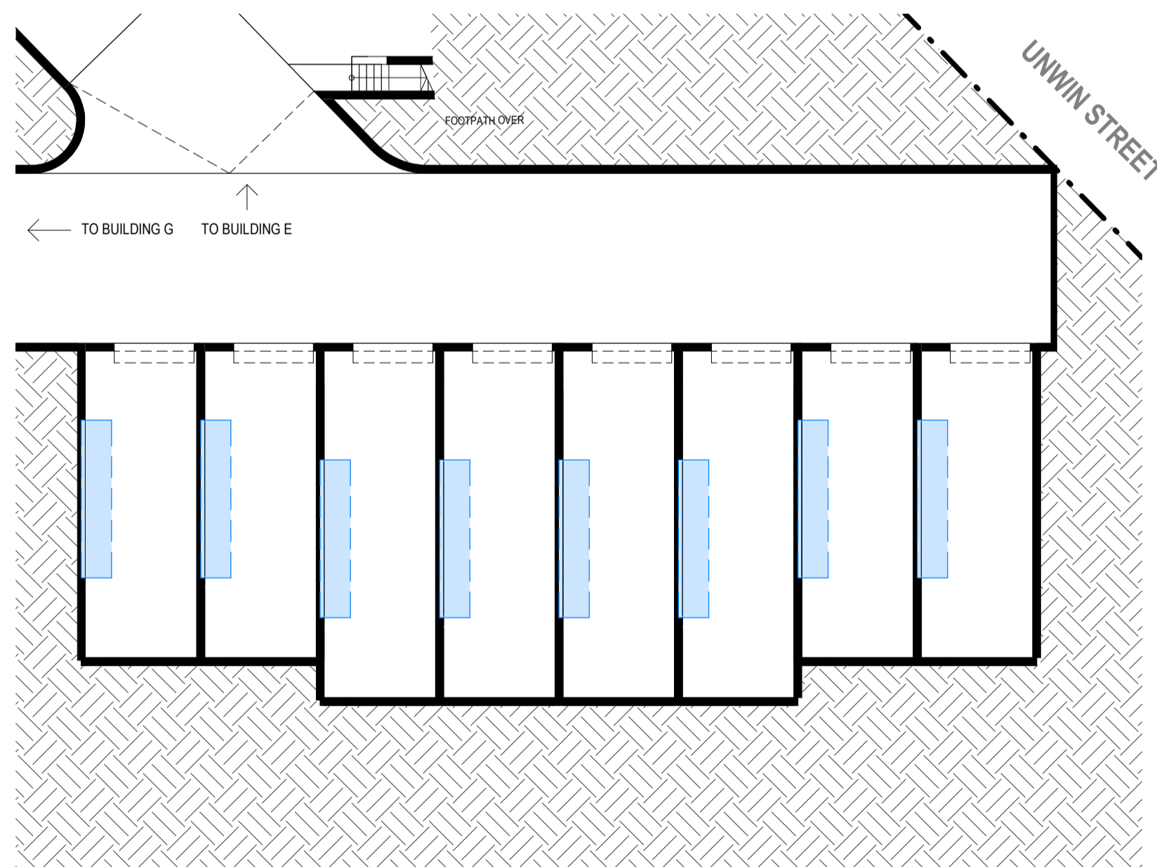
BUILDING F - UNDERCROFT (AREA) - PN
