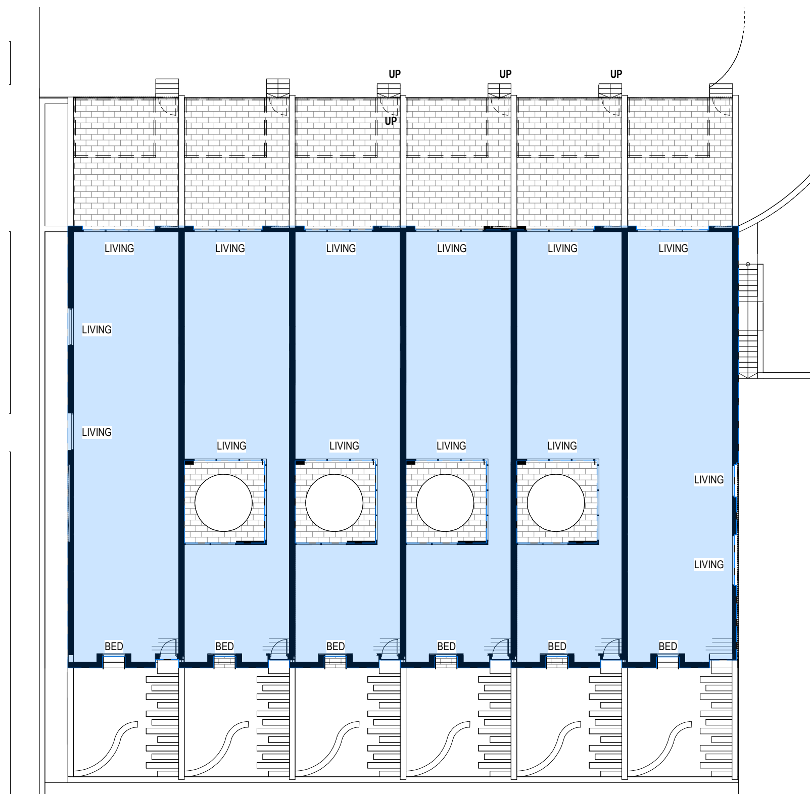
BUILDING J - GROUND FLOOR (AREA) - PN
