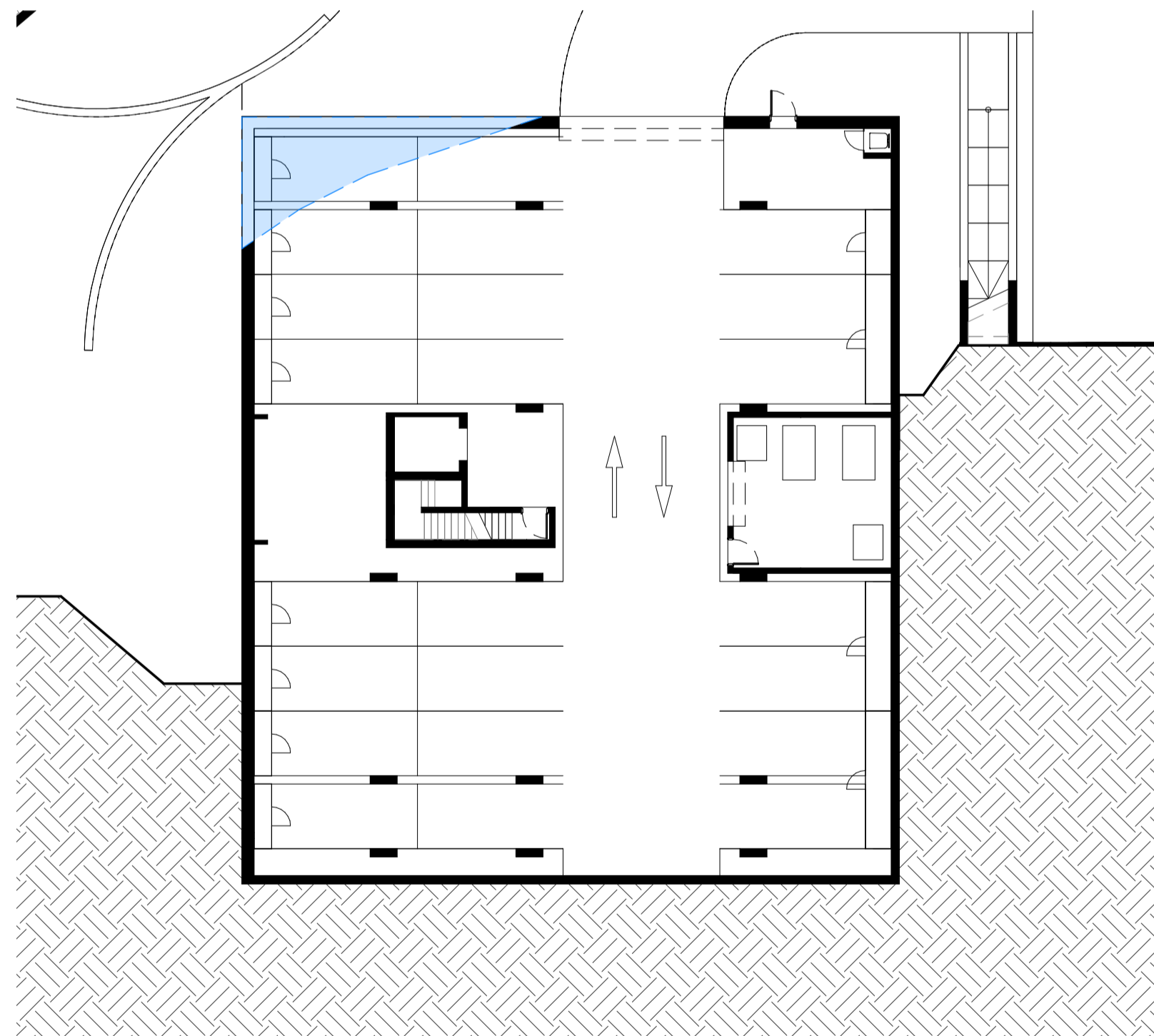
BUILDING K - UNDERCROFT (AREA) - PN
