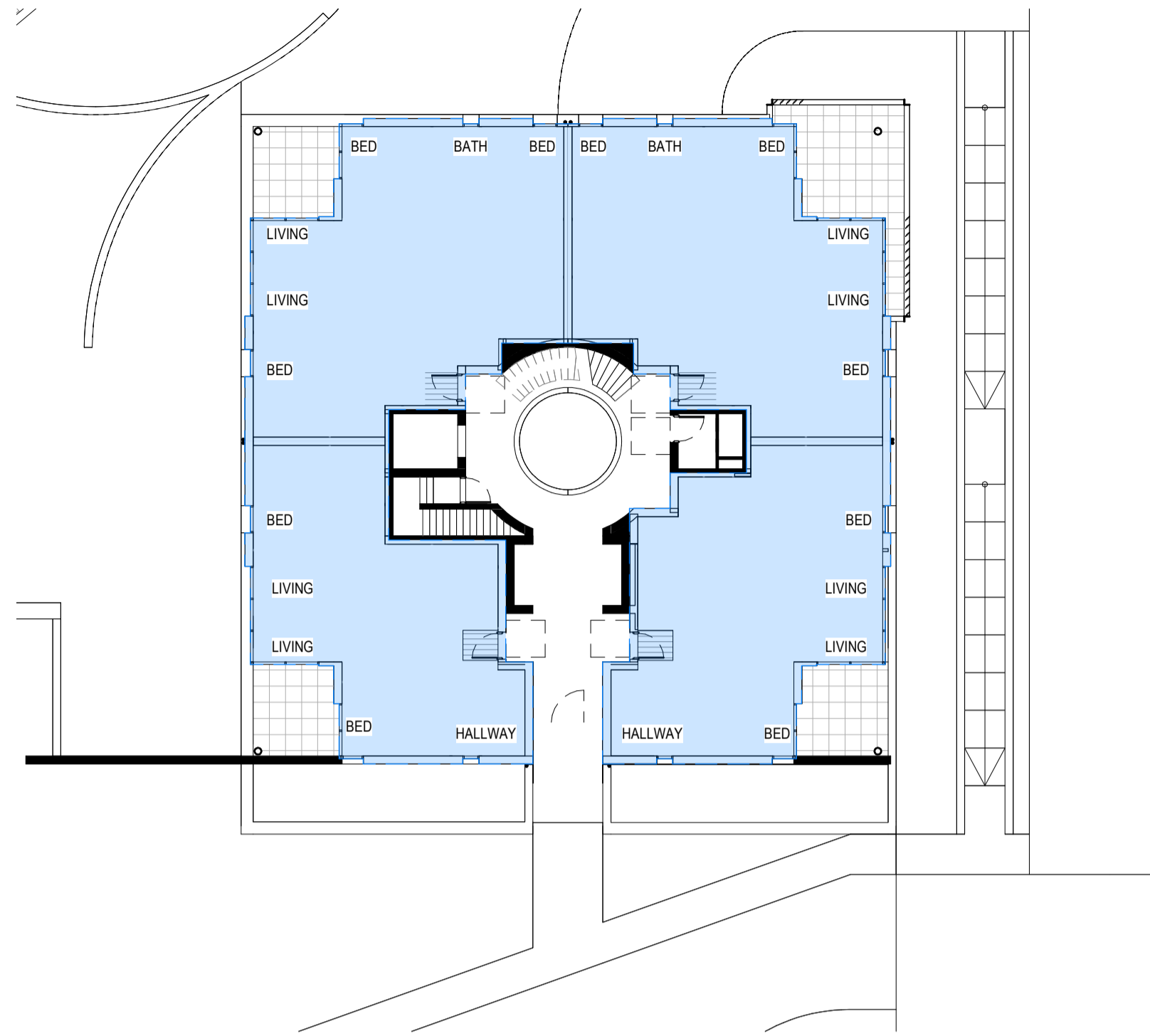
BUILDING K - GROUND FLOOR (AREA) - PN
