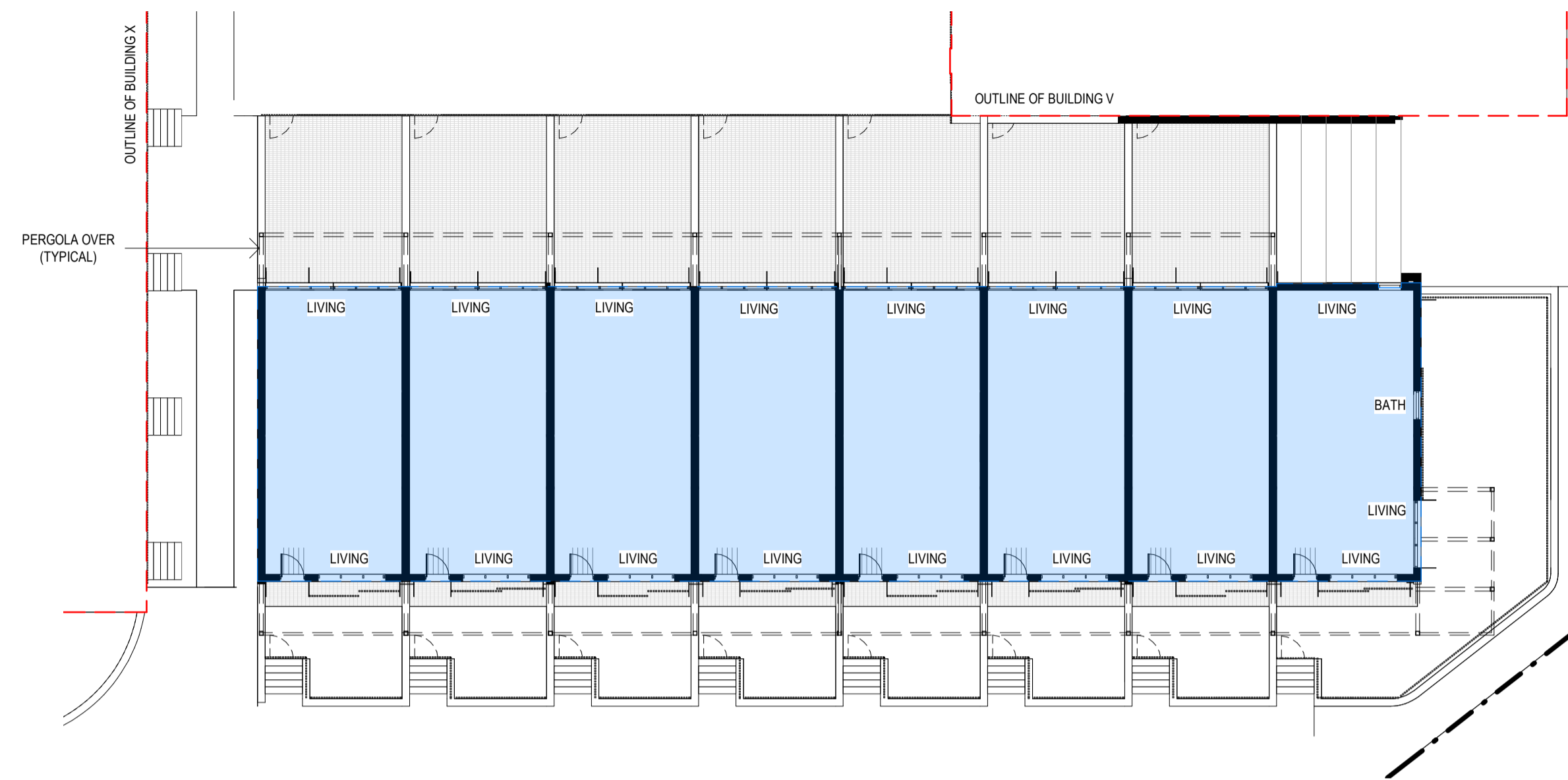
BUILDING W - GROUND FLOOR (AREA) - PN
