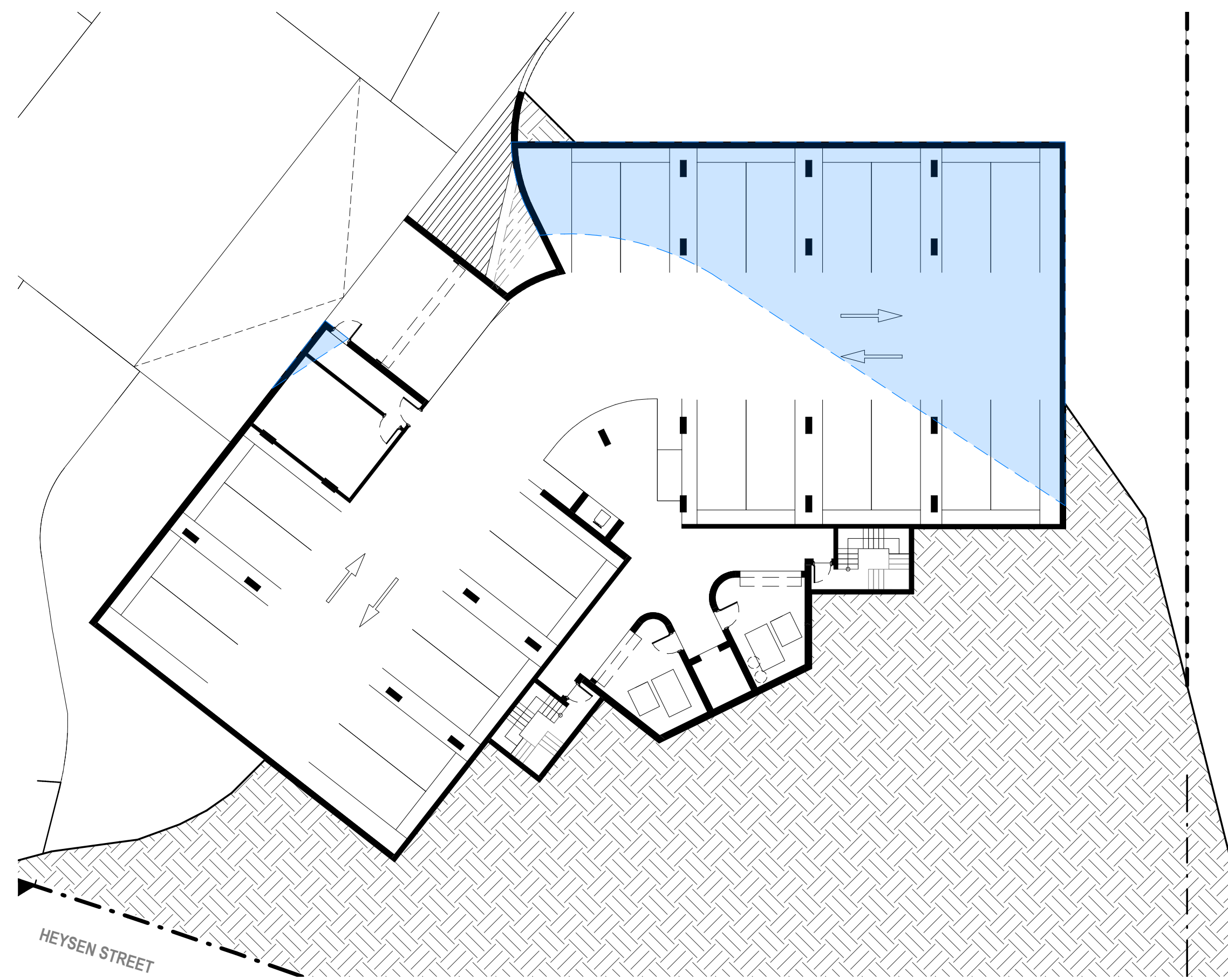
BUILDING Z - UNDERCROFT (AREA) - PN
