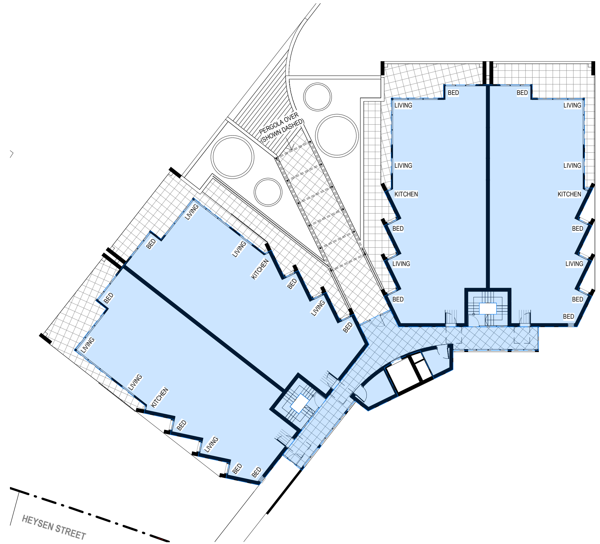
BUILDING Z - GROUND FLOOR (AREA) - PN
