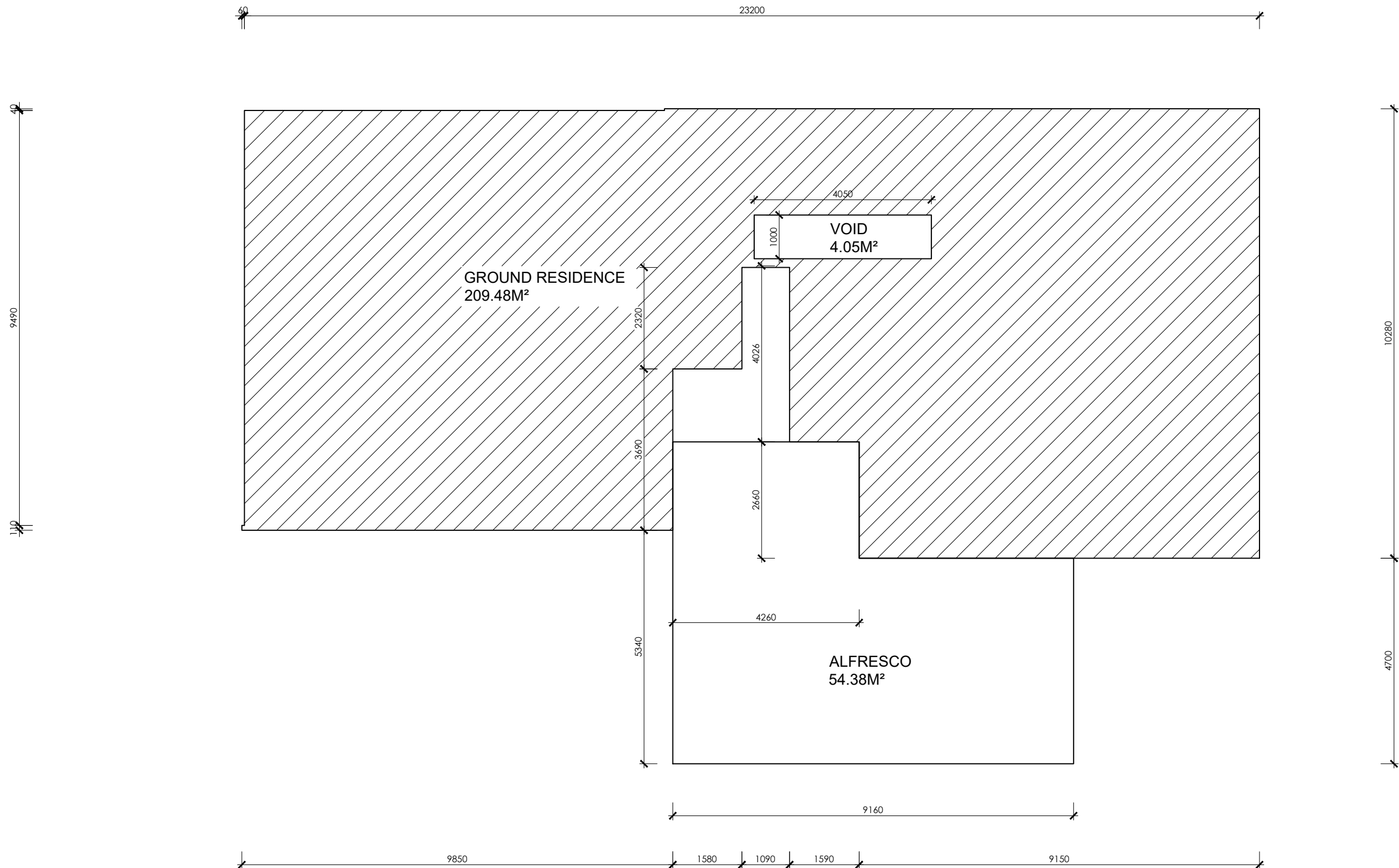
1 GROUND AREA PLAN
