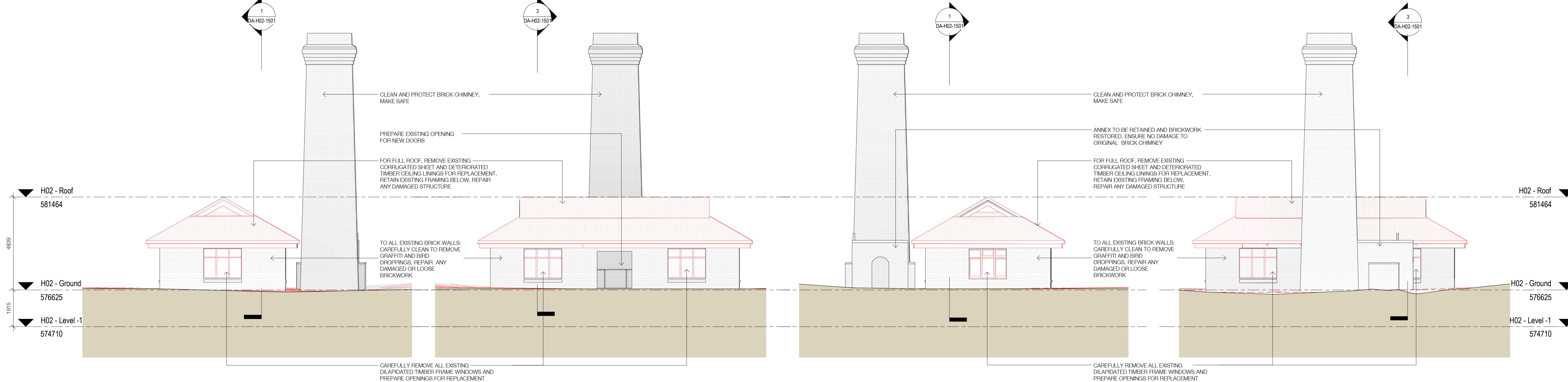
1 DA-H02 - Demolition Elevation - North 1: 100@A1
