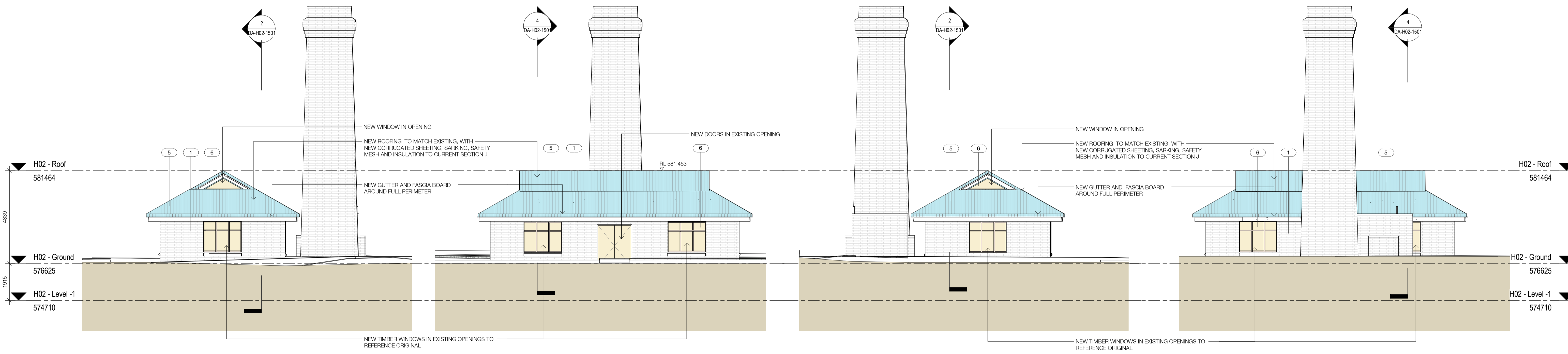
5 DA-H02 - Elevation North 1: 100@A1
