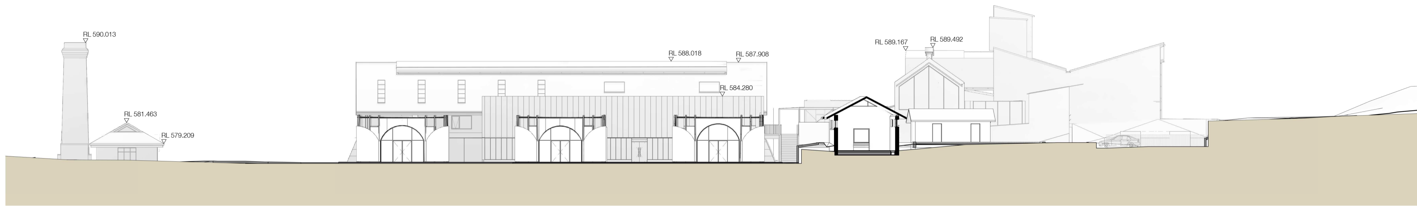
1 DA-H - Elevation South 1 : 250@A1
