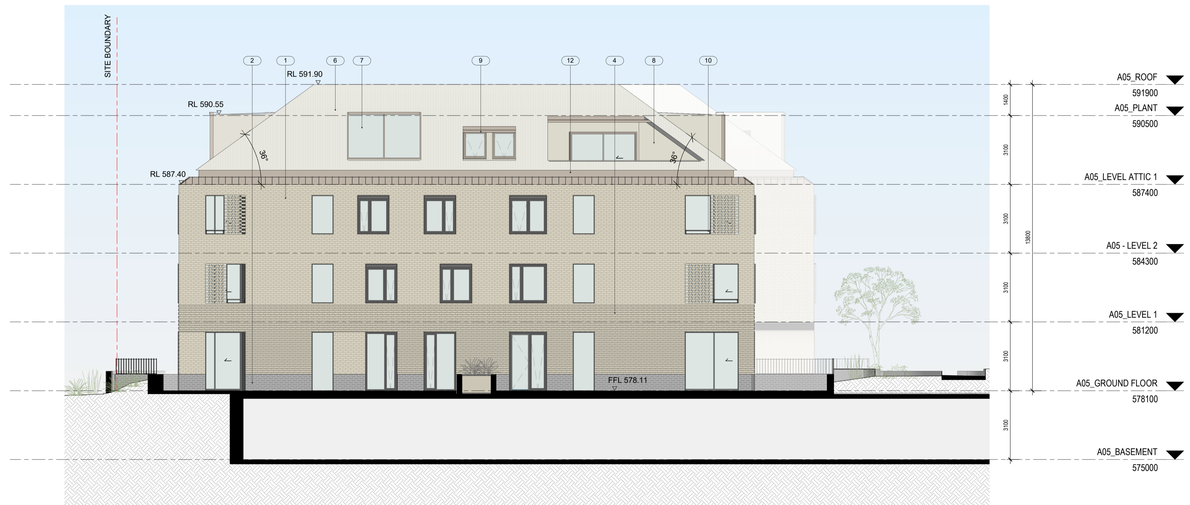
2 A05 - ELEVATION SOUTH DA-A-0251 1: 100@A1
