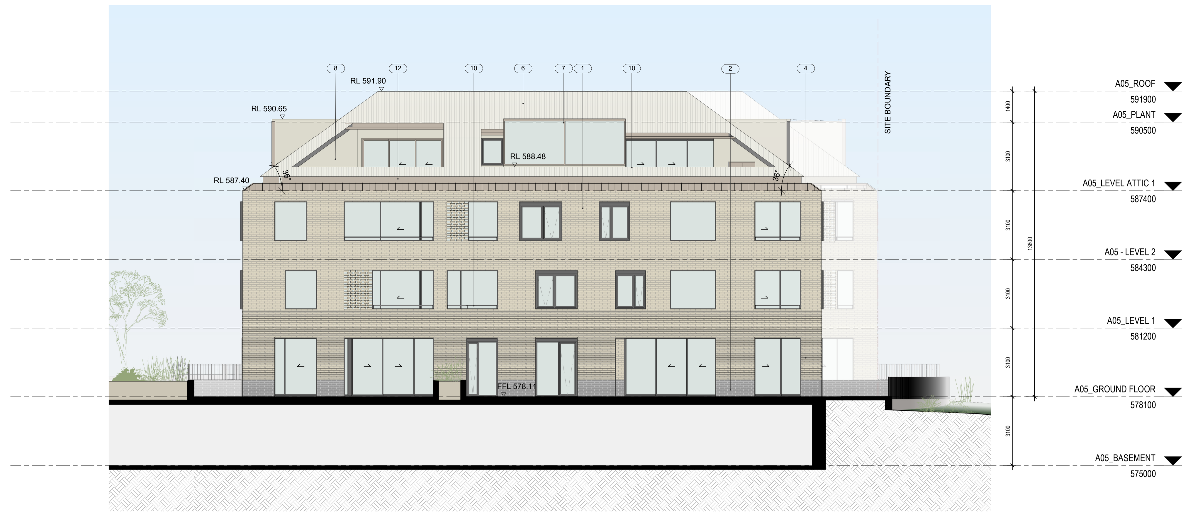
1 A05 - ELEVATION NORTH A-0-4441 1: 100@A1
