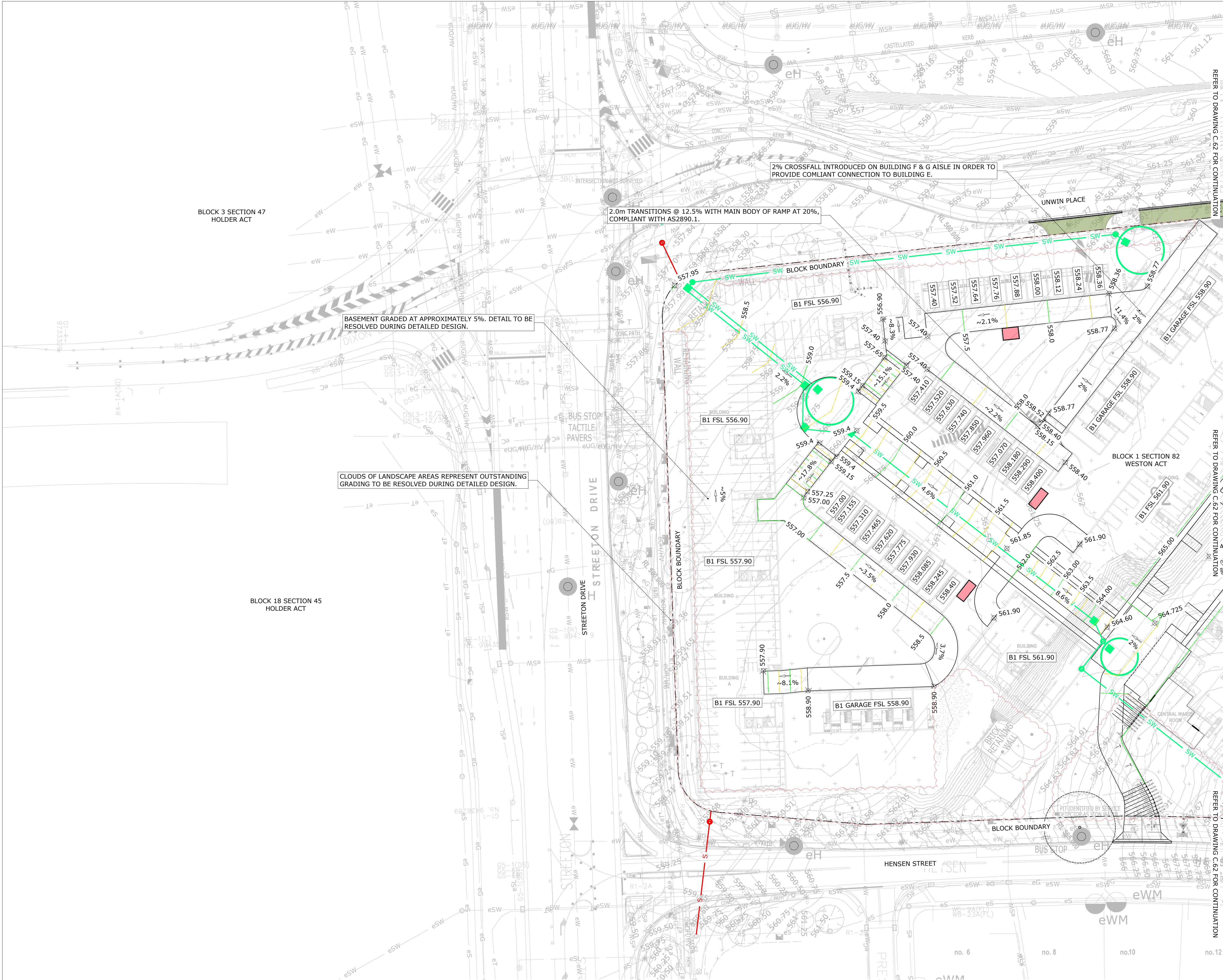
SITE GRADING PLAN (SHEET 01 OF 02) 1:500 @ A1
