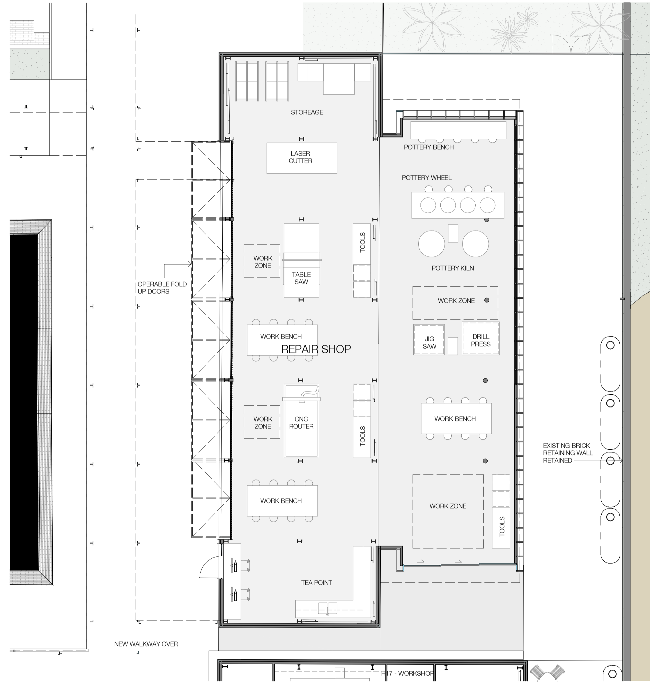
H16 MACHINE BAY II REPAIR SHOP 295m 2
