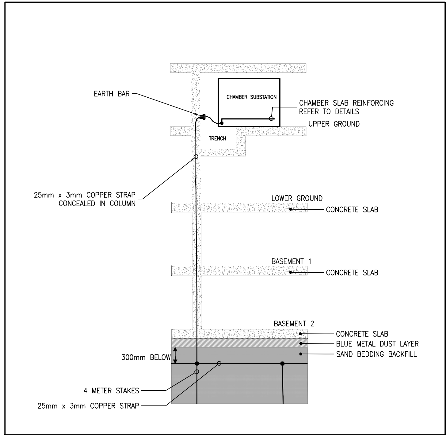
SECTION DETAIL 1 : EARTH MATT DEPTH OF INSTALLATION SECTION N.T.S
