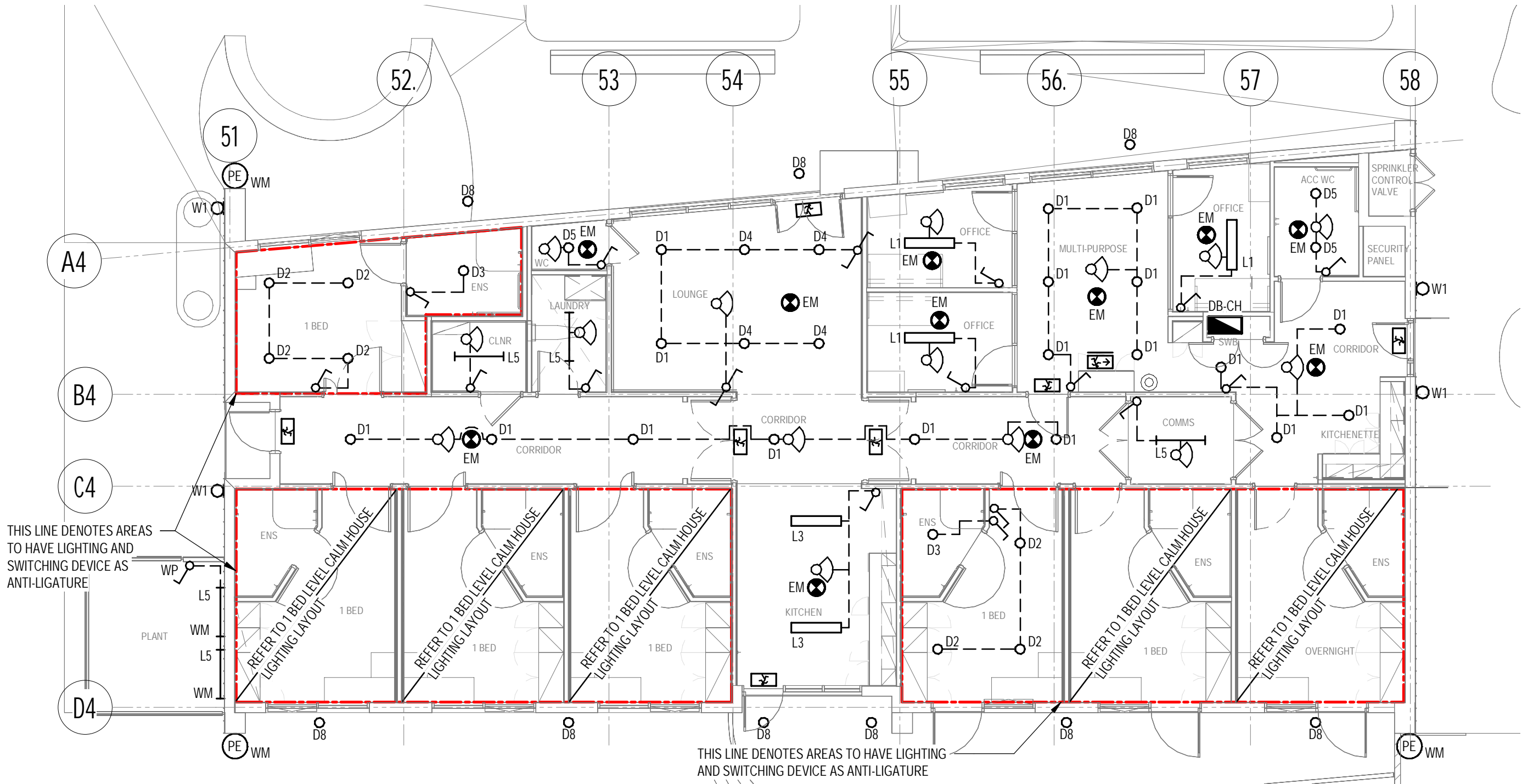
GROUND LEVEL - CALM HOUSE LIGHTING LAYOUT 1 : 100
