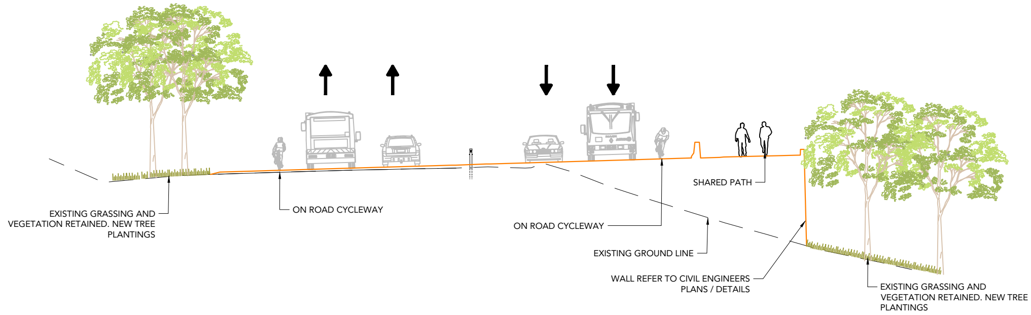
E SECTION: CHAINAGE 4080 (REFER CIVIL FOR LOCATION) SCALE: 1:200@A3
