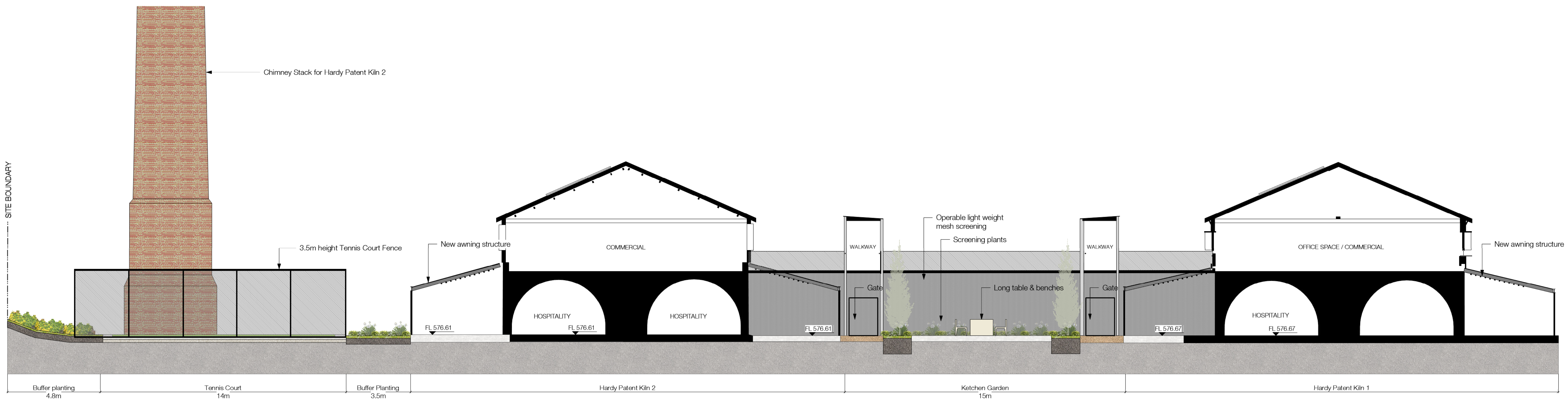
1 East Section - Kitchen Garden Section - Scale 1:100
