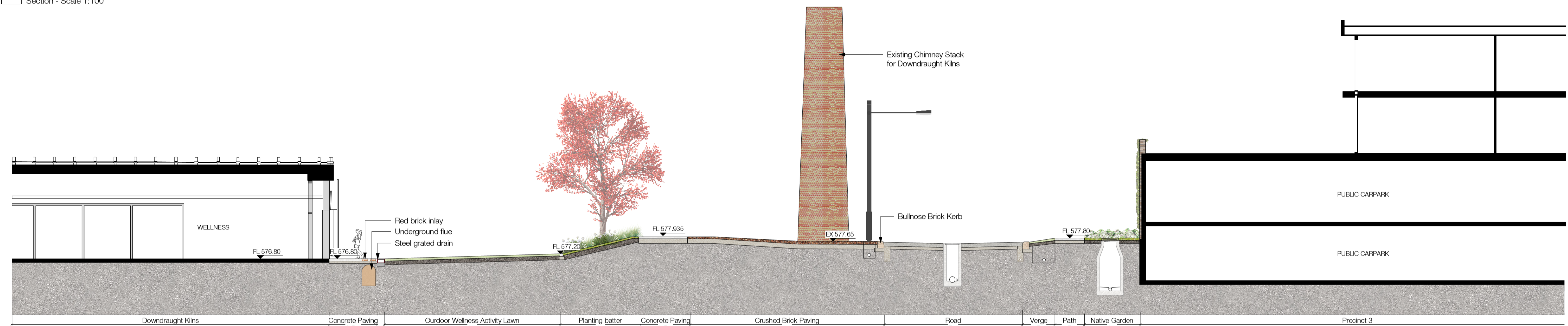
2 East Section - Wellness Center Section - Scale 1:100
