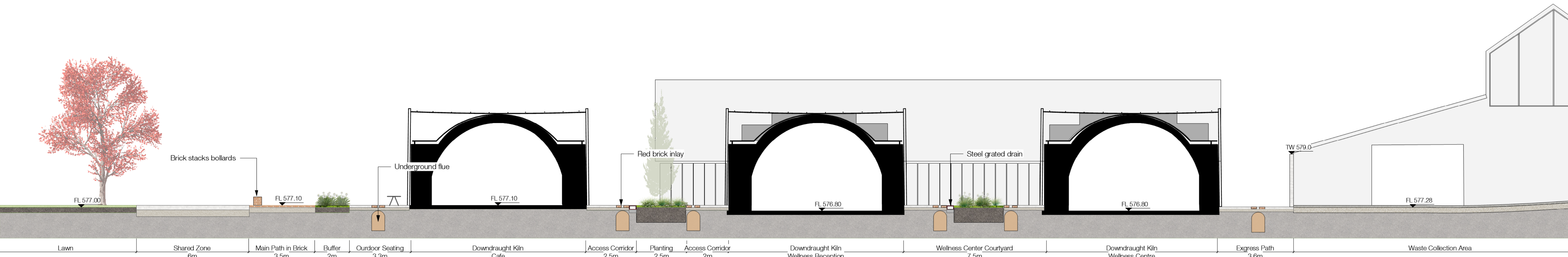
1 North Section - Downdraught Kiln Section - Scale 1:100
