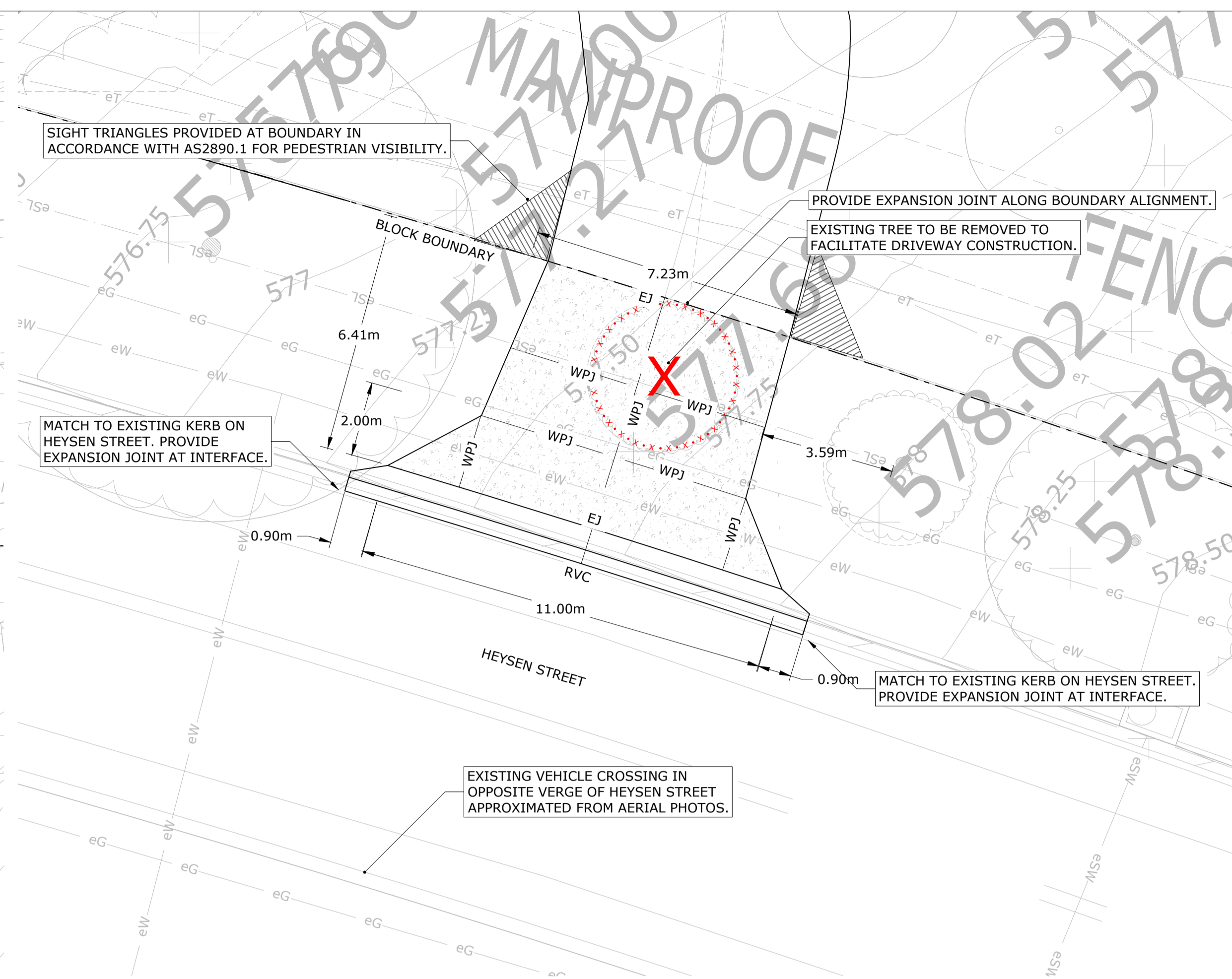
PROPOSED DRIVEWAY SET OUT PLAN - HEYSEN STREET (EAST) - DRIVEWAY 2 1:100 @ A1
