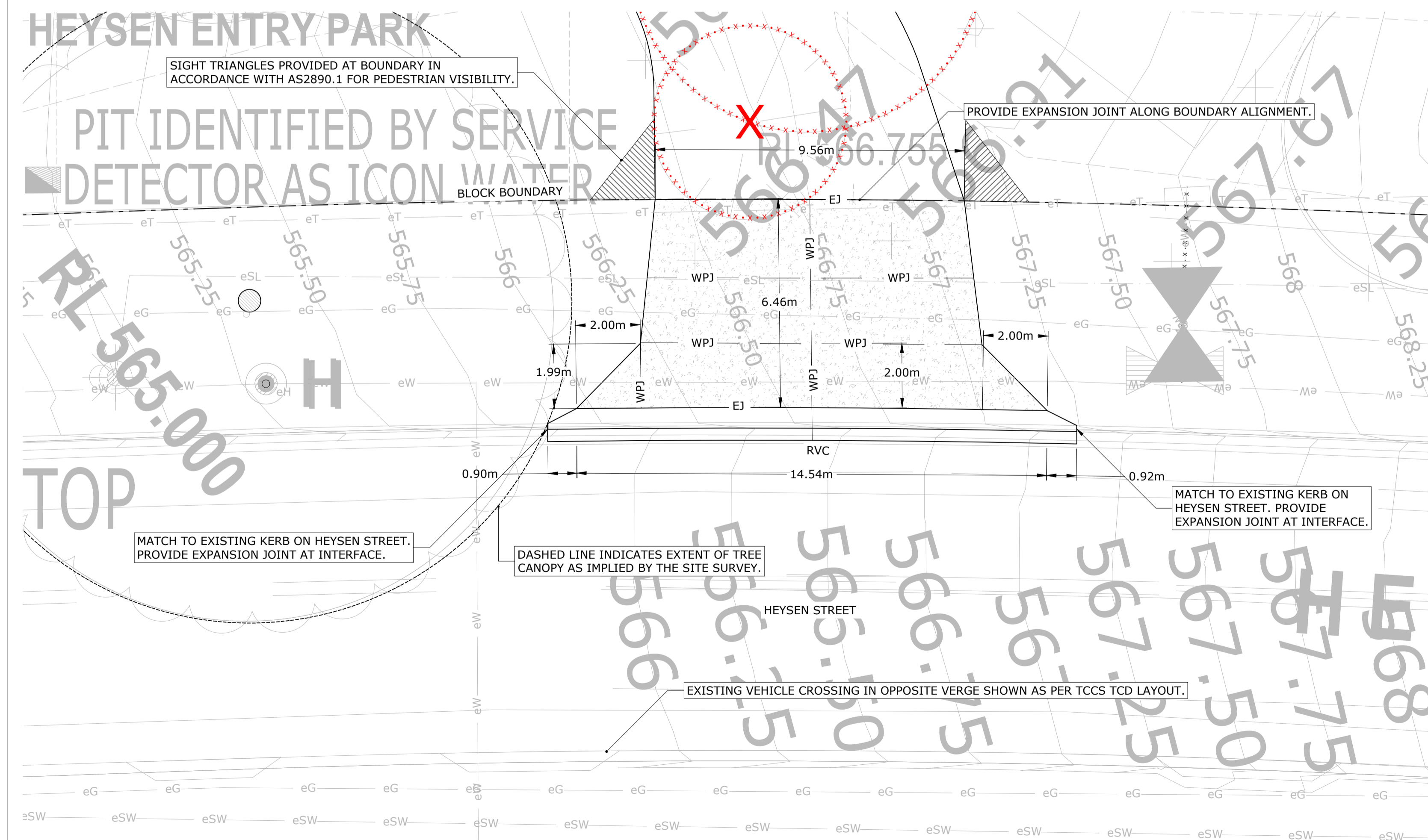
PROPOSED DRIVEWAY SET OUT PLAN - HEYSEN STREET (WEST) - DRIVEWAY 3 1:100 @ A1
