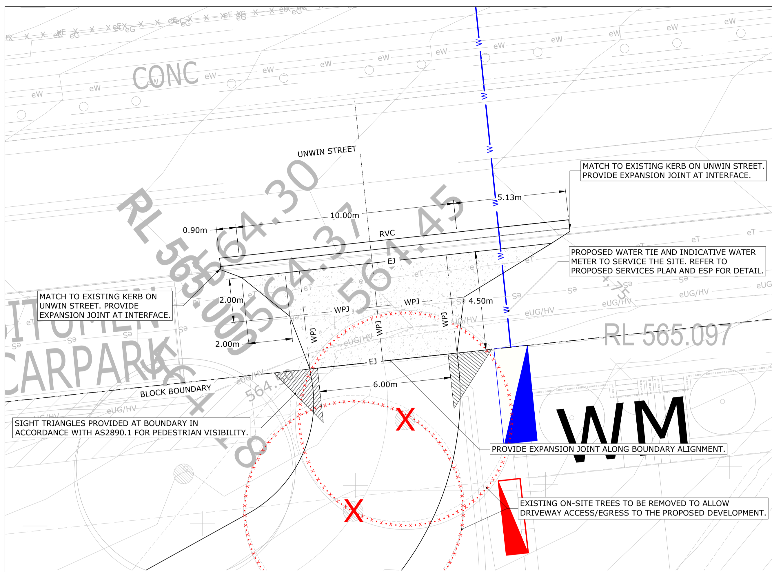
PROPOSED DRIVEWAY SET OUT PLAN - UNWIN STREET - DRIVEWAY 1 1:100 @ A1
