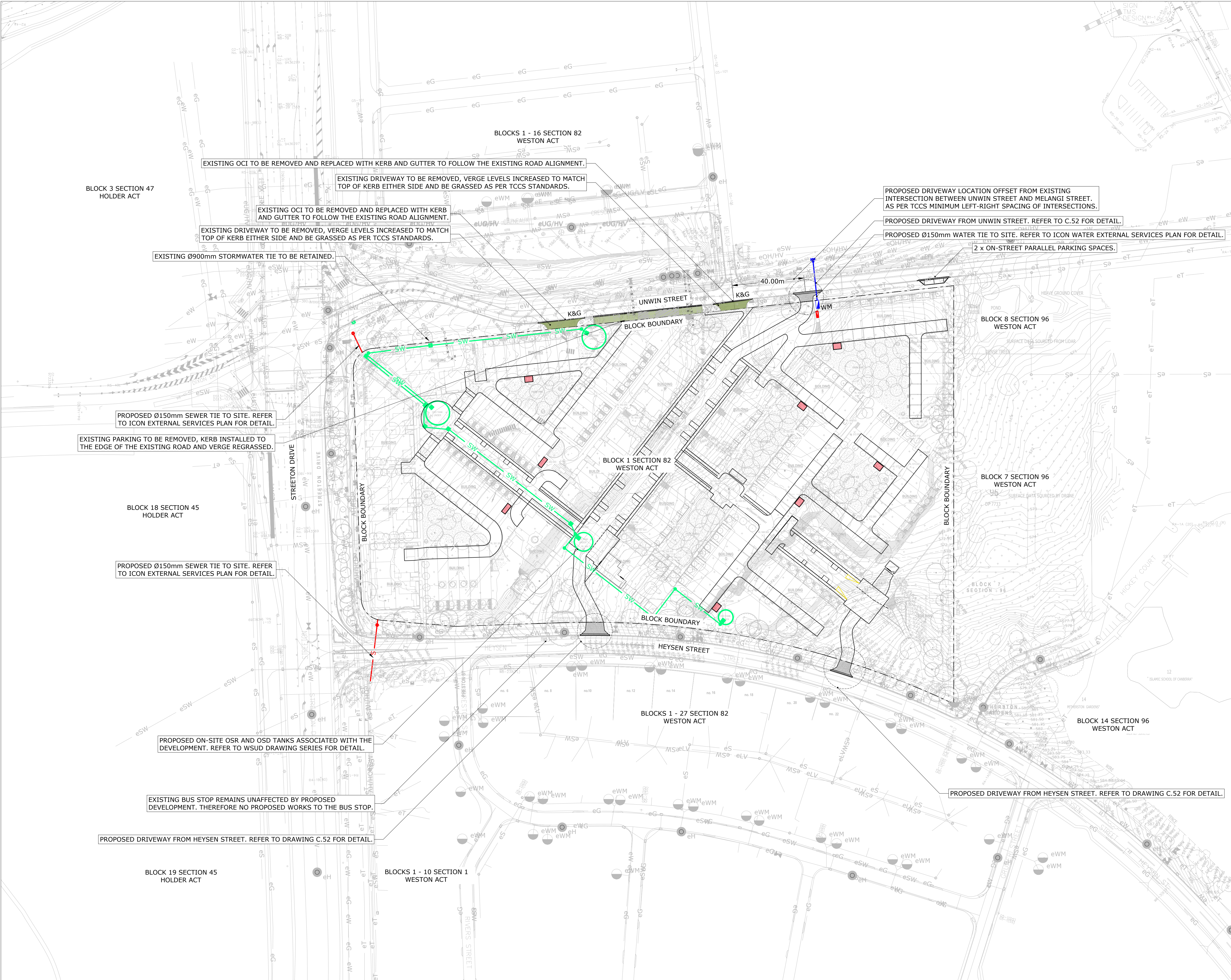
VERGE WORKS - GENERAL ARRANGEMENT PLAN 1:1000 @ A1
