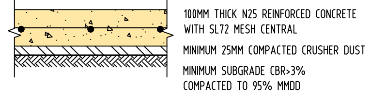
FOOTPATH DETAIL
