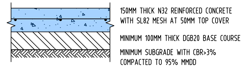
CONCRETE PAVEMENT - 150mm
