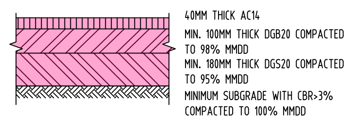
ASPHALT PAVEMENT
