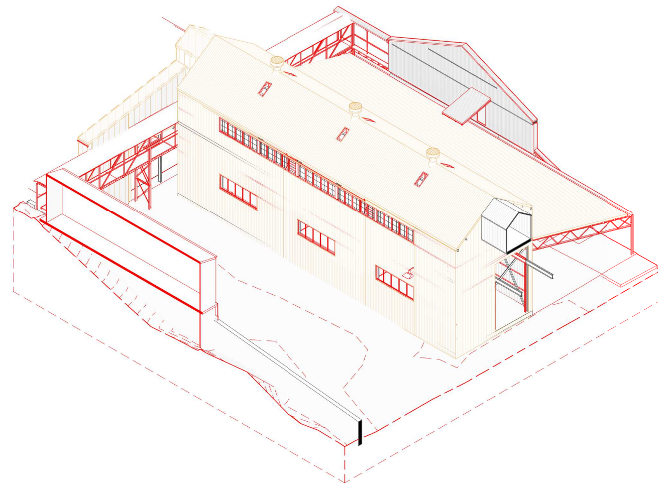
1 H16 - Existing/Demolition - NE View @A1
