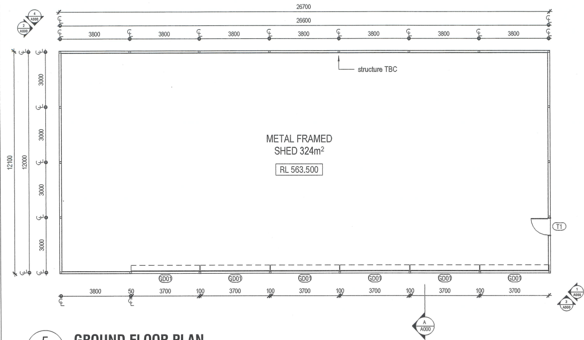
5 GROUND FLOOR PLAN SCALE 1:100 @A1
