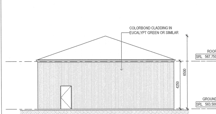
1 ELEVATION 01 SCALE 1:100 @A1
