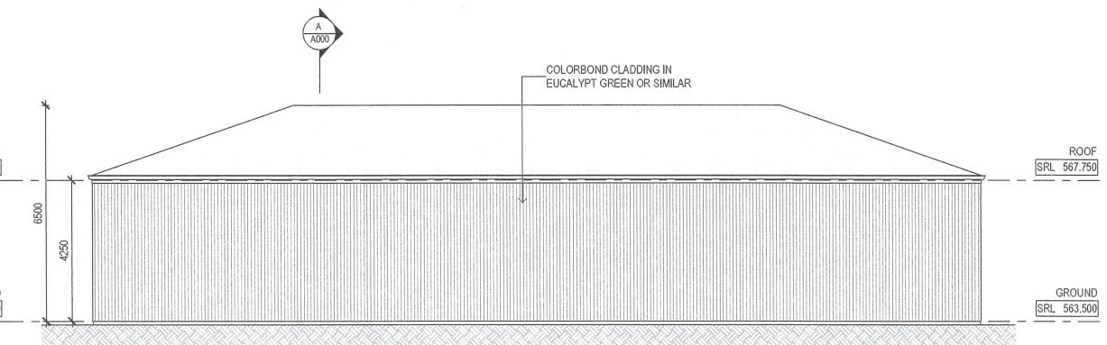
4 ELEVATION 04 SCALE 1:100 @A1
