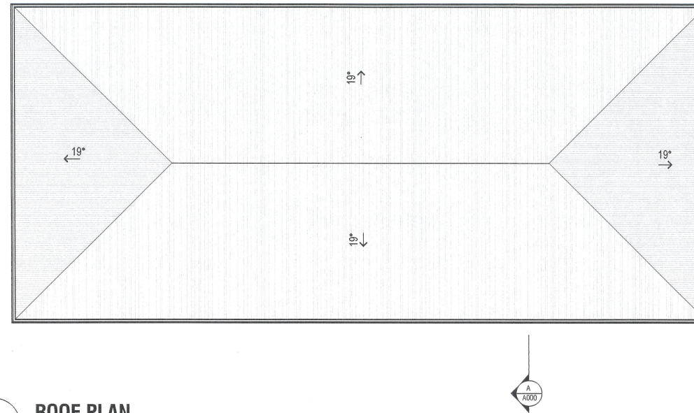
6 ROOF PLAN SCALE 1:100 @A1
