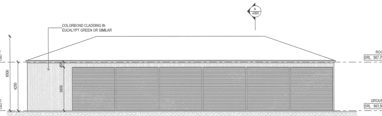
3 ELEVATION 03 SCALE 1:100 @A1
