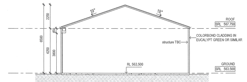
A SECTION A SCALE 1:100 @A1
