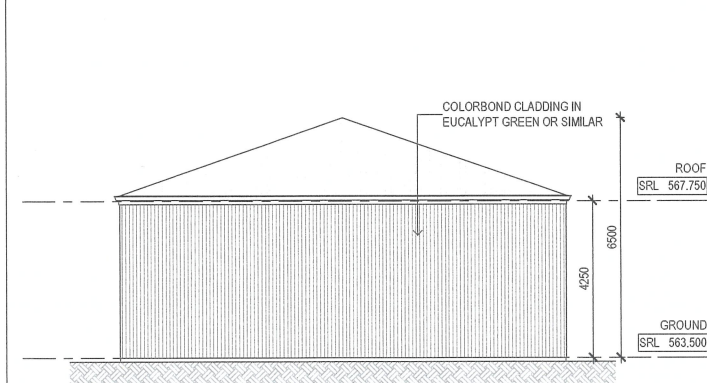
2 ELEVATION 02 SCALE 1:100 @A1
