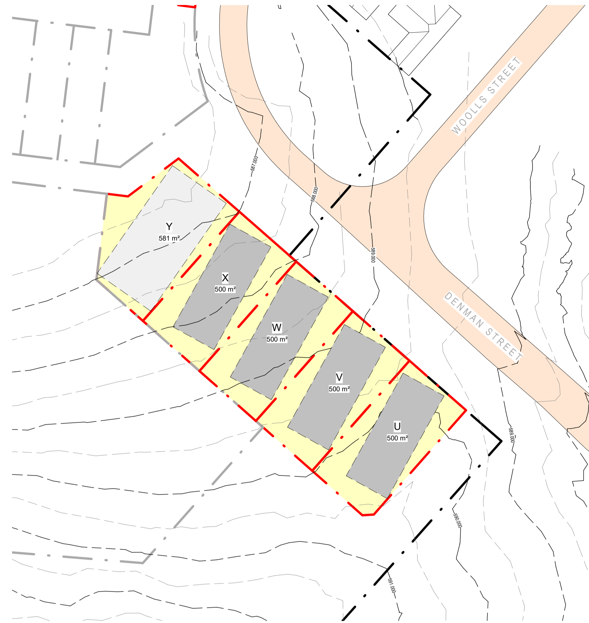
BLOCK COMPLIANCE PLAN - LOTS T1 - T5
