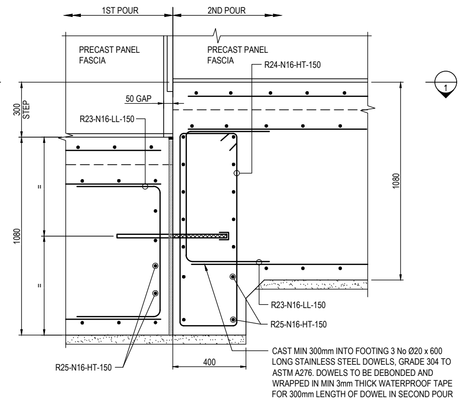
TYPICAL PANEL FOOTING STEP WITH EXPANSION JOINT (EJP)
