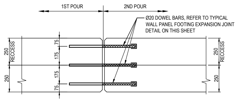
SECTION 1 SCALE 1:10
