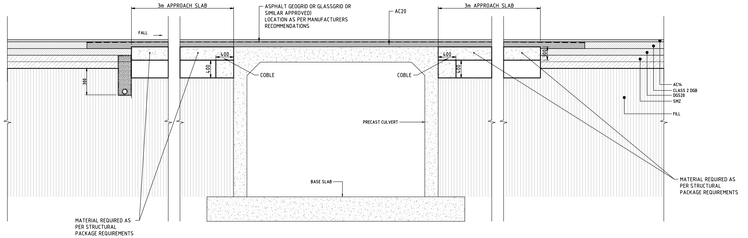
UNDERPASS CH 4588
