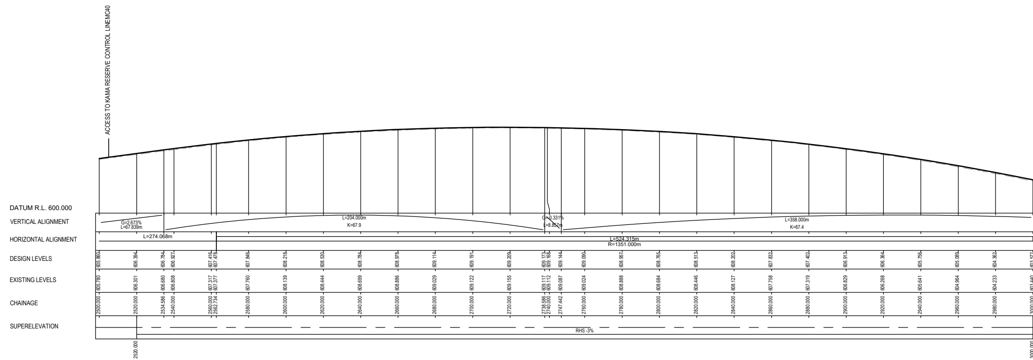
LONGITUDINAL SECTION ALONG CONTROL MC00 HORIZONTAL 1 : 1000 VERTICAL 1 : 200
