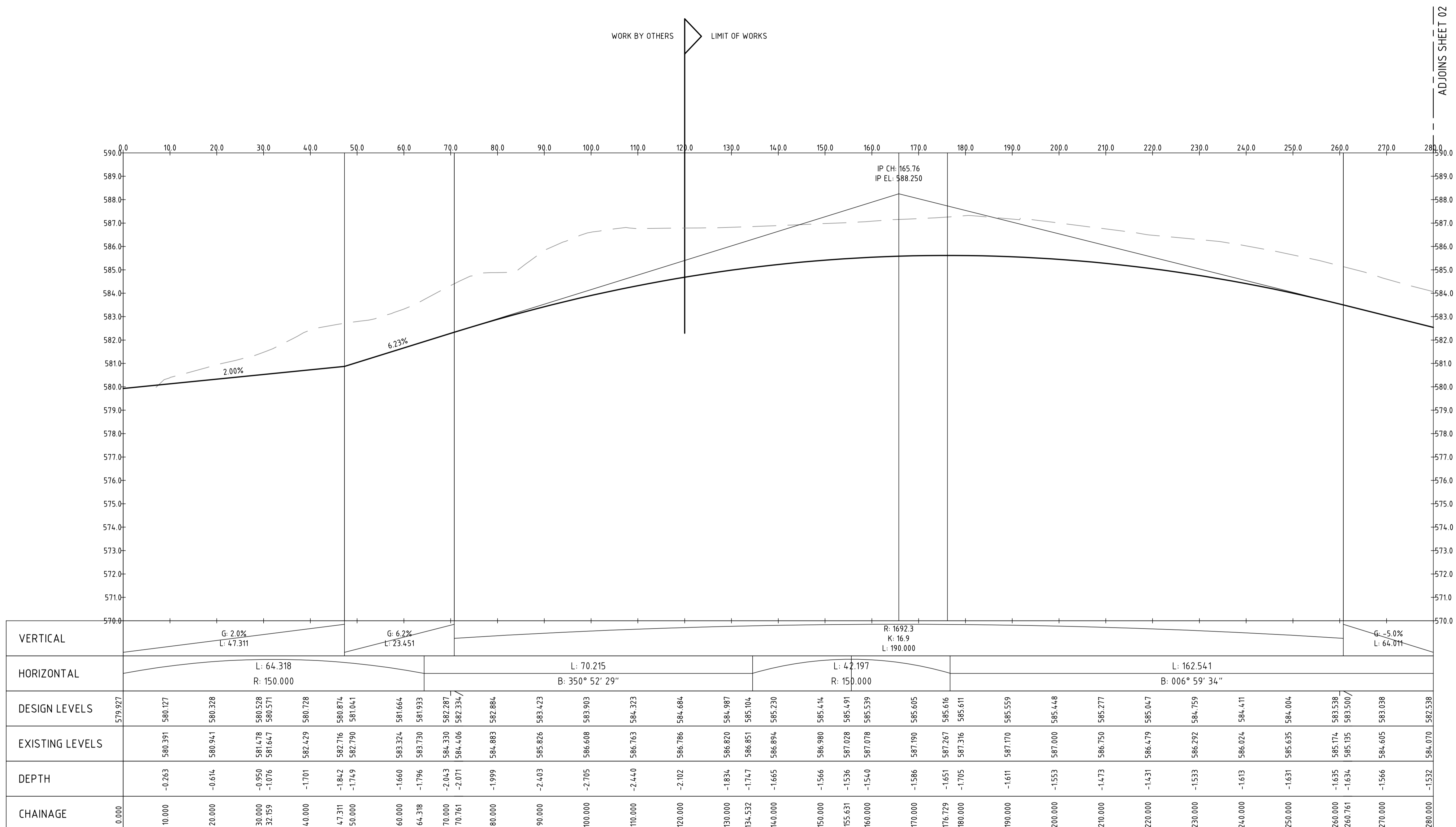
PROFILE OF ALIGNMENT AL-01 (VERT SCALE 1:100, HOR SCALE 1:500, VERT EXAG 1:5) FROM: CH 0.000 TO CH 280.000
