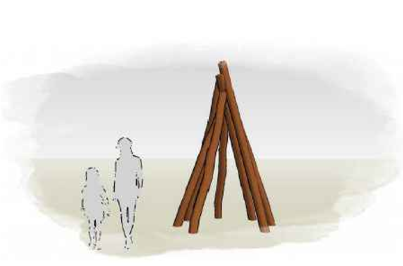
2 PROPRIETARY FURNITURE: TEEPEE RUSTIC SCALE: NTS MANUFACTURER: Lypa CODE: L001002 SLATS: Timber DIMENISON: 3000mm H x 2300mm D INSTALLATION: Subsurface, to manufacturer's specification
