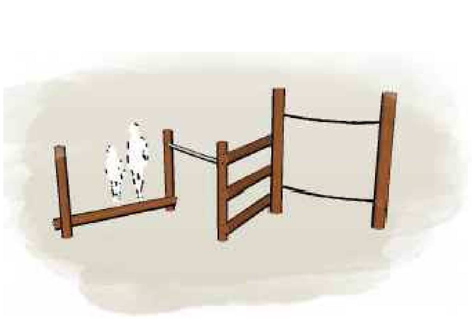
4 PROPRIETARY FURNITURE: SPARROW TRAIL SCALE: NTS MANUFACTURER: Lypa CODE: L021100 SLATS: Timber DIMENISON: 5650mm L x 2500mm W x 2400mm H INSTALLATION: Subsurface, to manufacturer's specification
