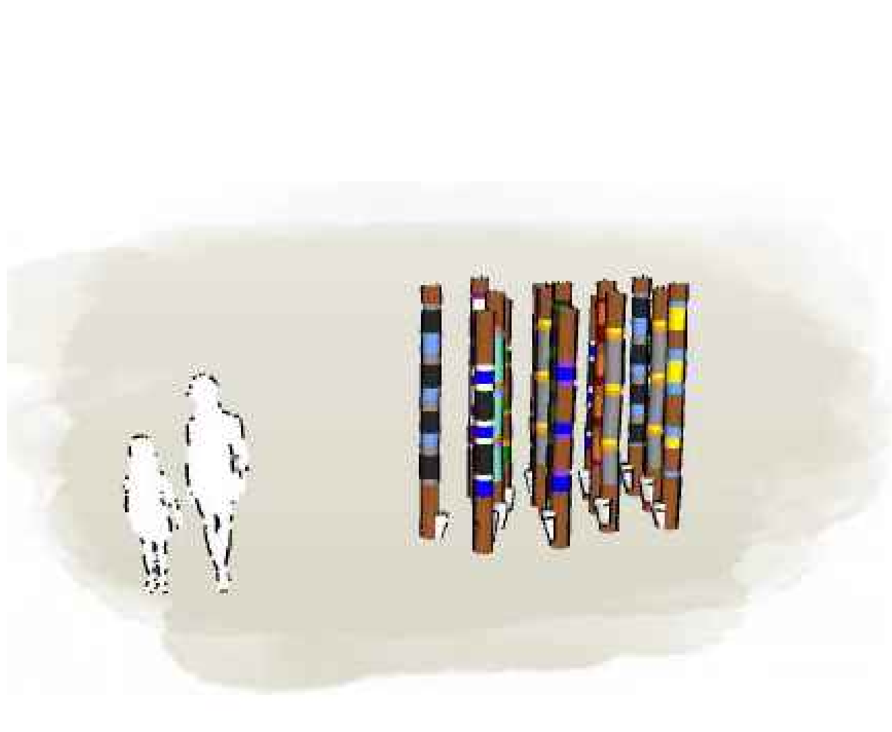
3 PROPRIETARY FURNITURE: CLUSTER CLIMBER SCALE: NTS MANUFACTURER: Lypa CODE: L004000 SLATS: Timber DIMENISON: 1800mm L x 300-500mm H x 2600mm L x 2200mm H INSTALLATION: Subsurface, to manufacturer's specification
