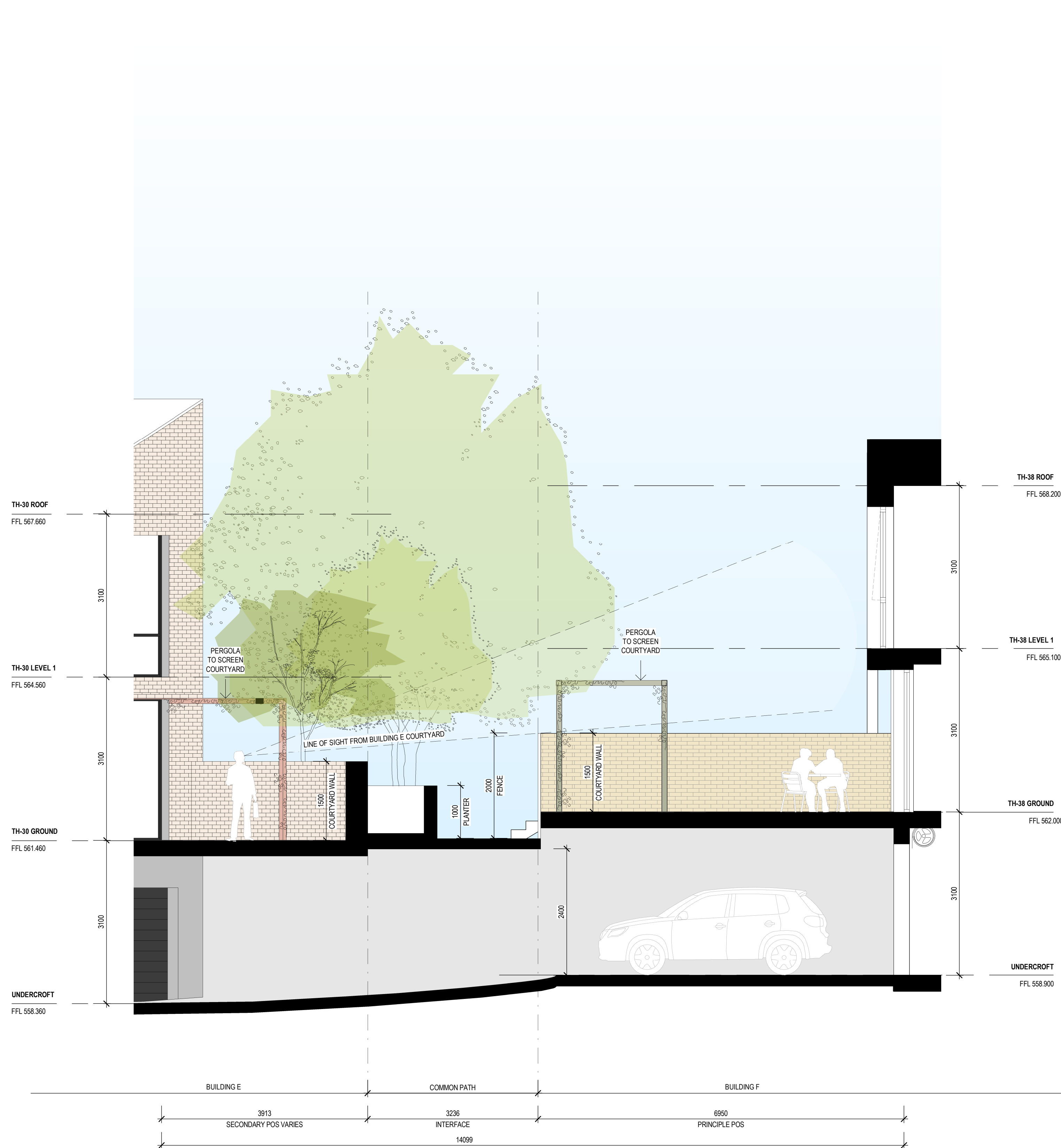
1 SECTION - INTERFACE BUILDINGS E & F
