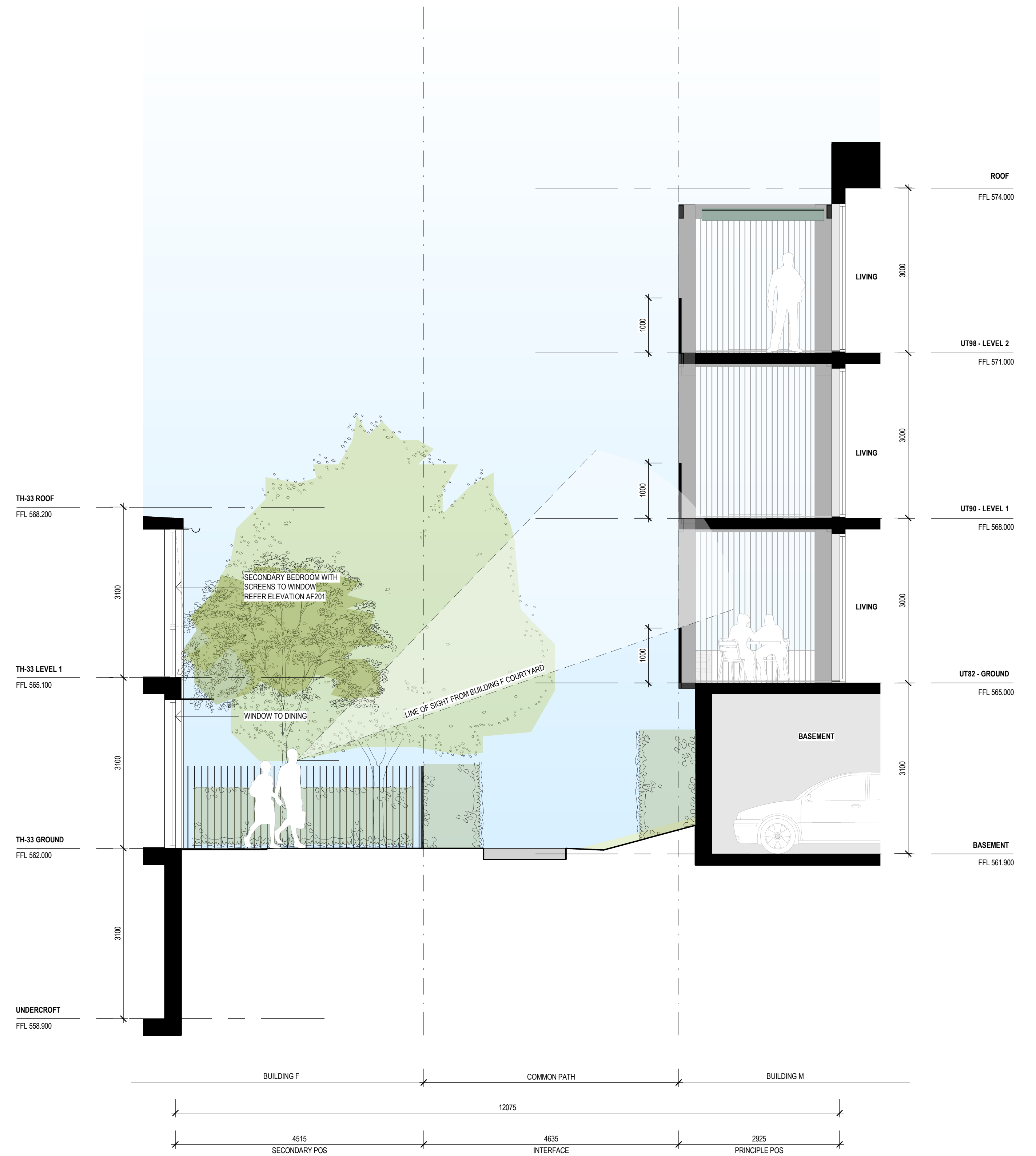
2 SECTION - INTERFACE BUILDINGS F & M NOTE: BUILDING F PPDS & LIVING ROOM ON NORTHERN FACADE
