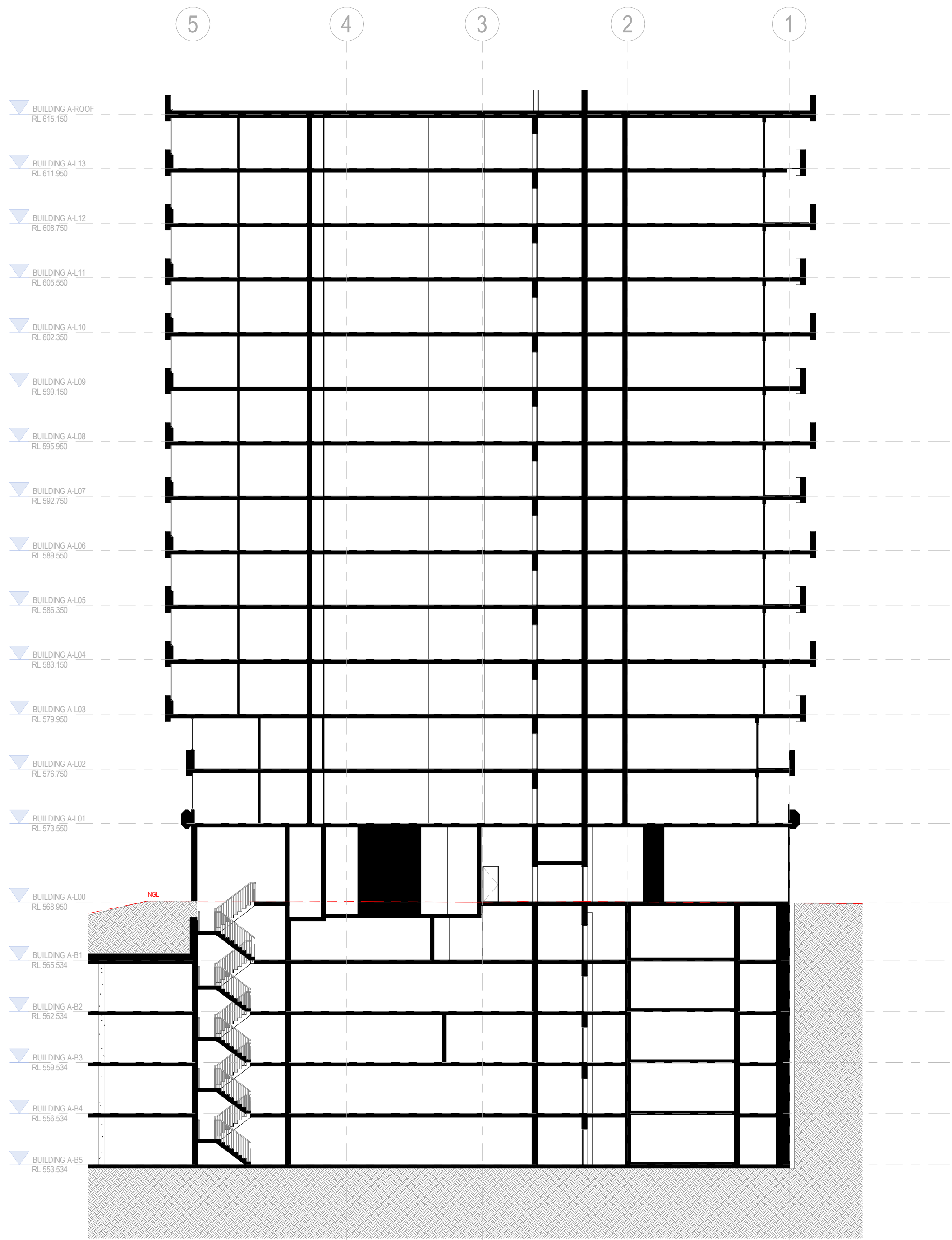
1 BUILDING A SHORT SECTION 3 1 : 200
