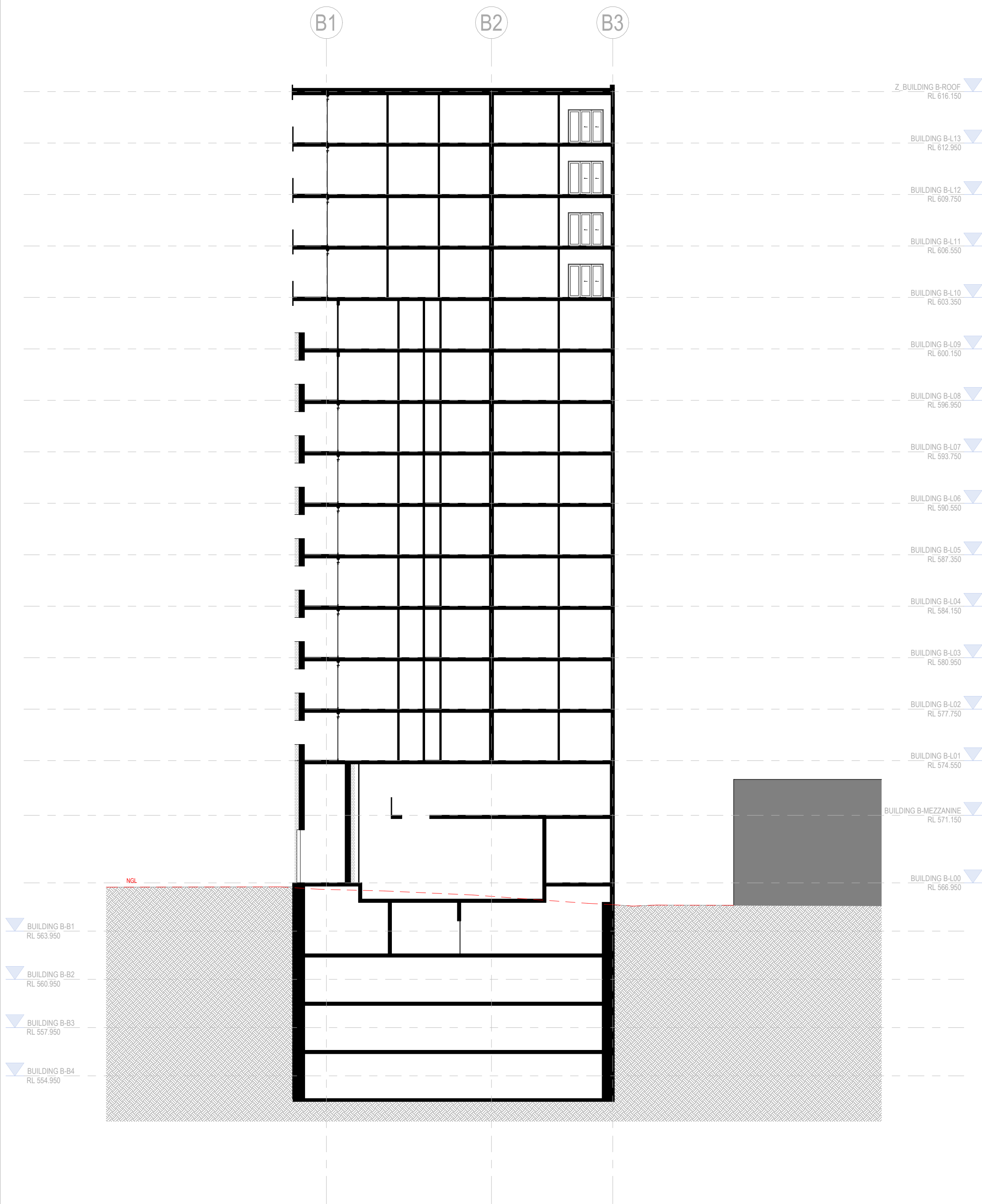
1 BUILDING B SHORT SECTION 1 1 : 200
