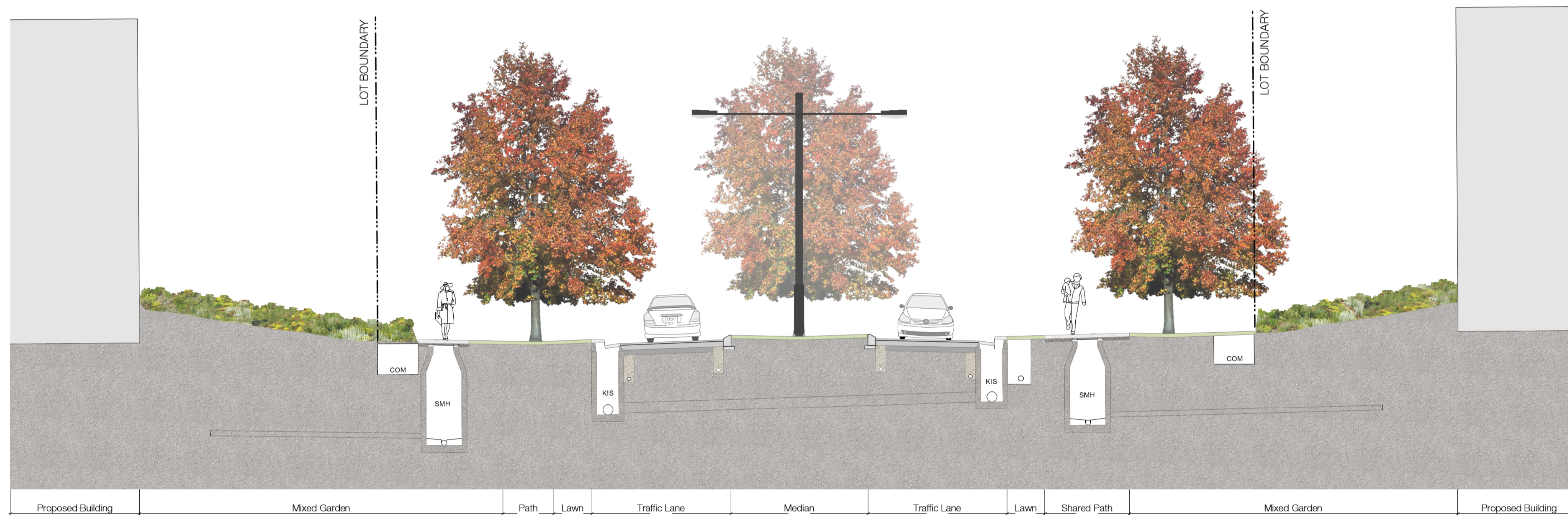
1 Quarr Drive Typical Section Section - Scale 1:80
