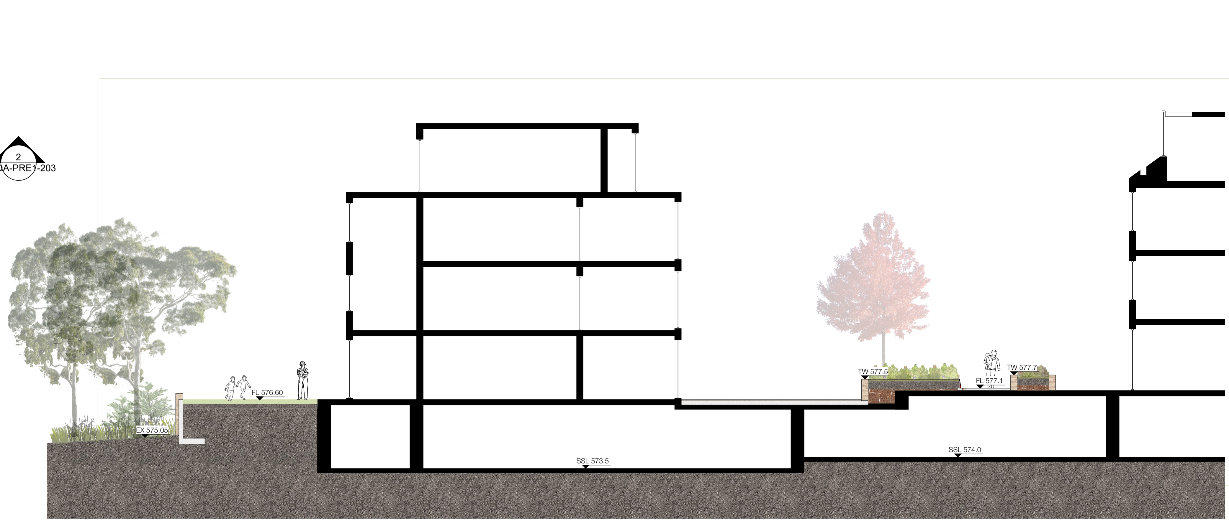
2 Section through A04 Section - Scale 1:100
