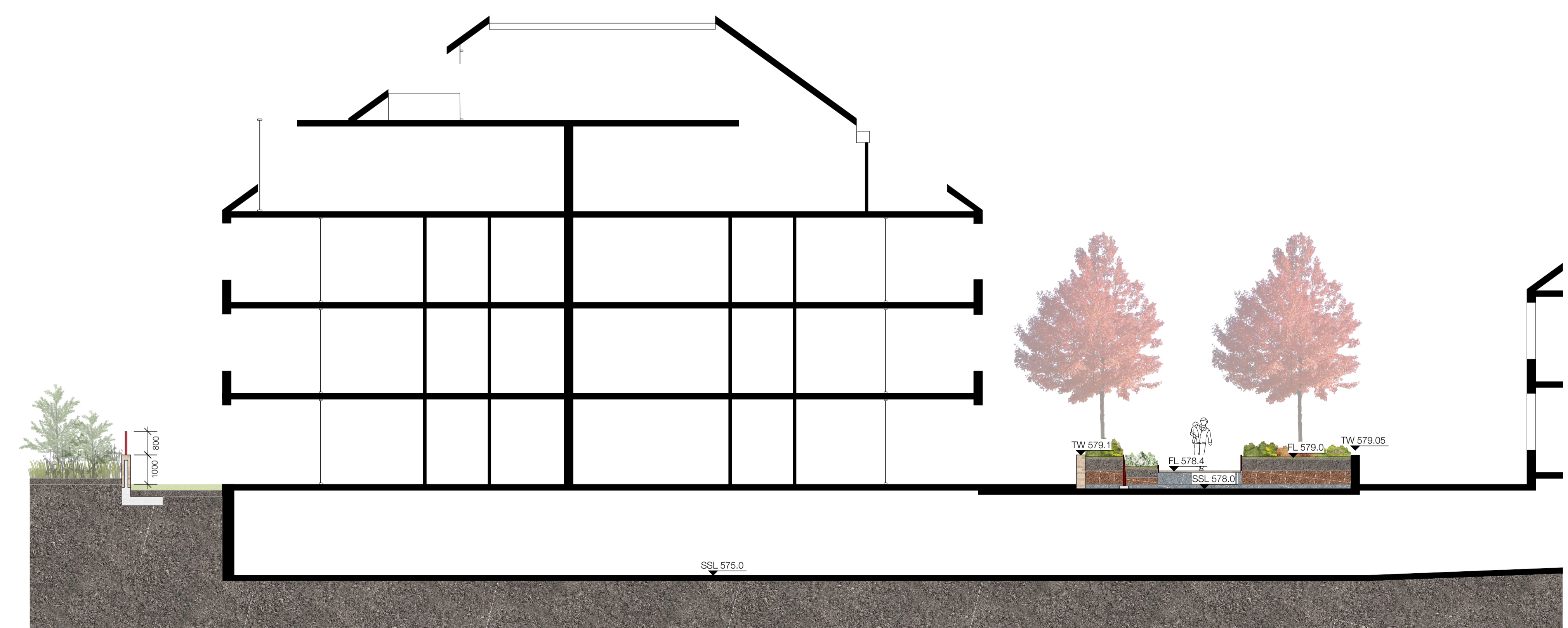
3 Section through A05 Section - Scale 1:100
