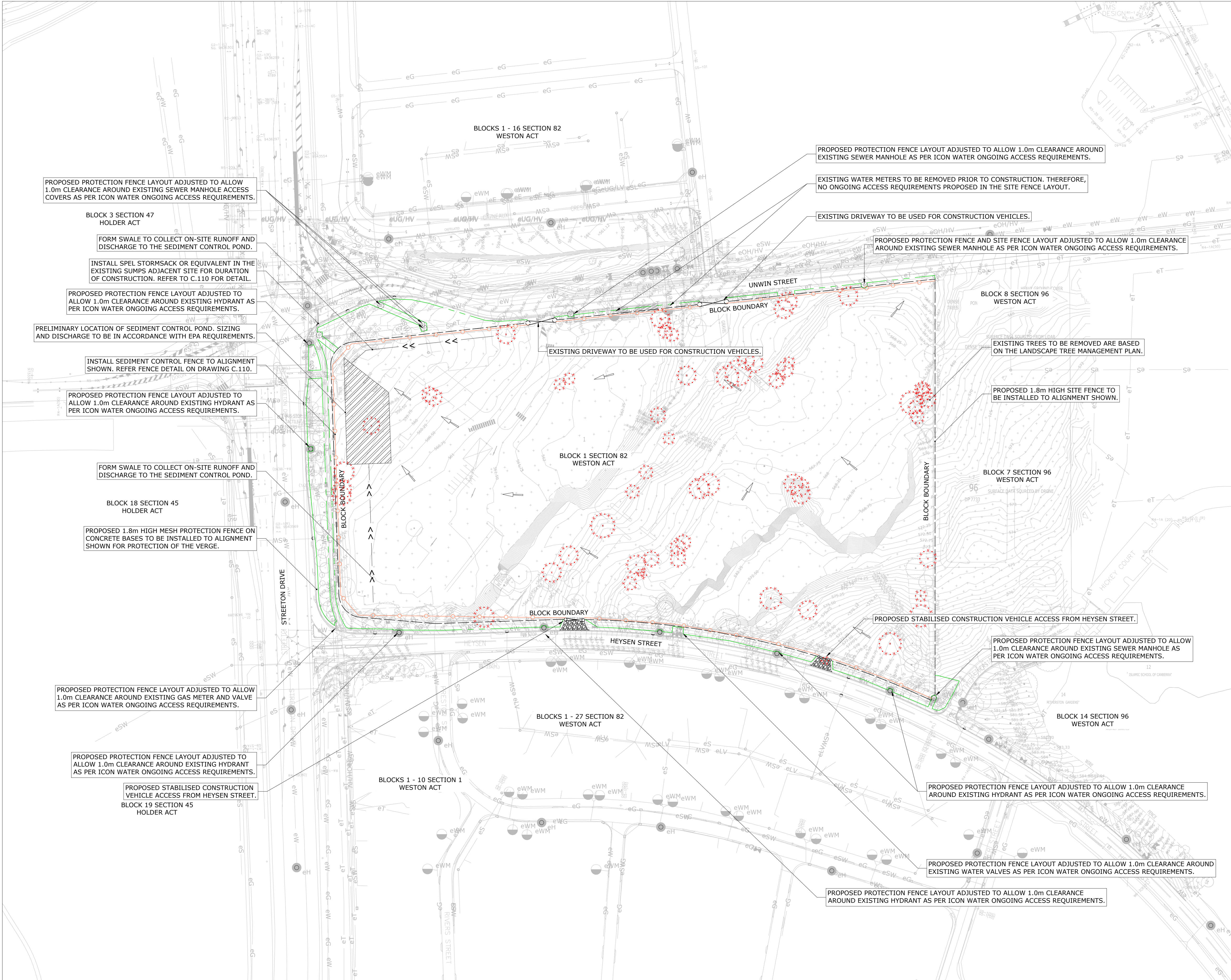
SEDIMENT AND EROSION CONTROL PLAN 1:1000 @ A1
