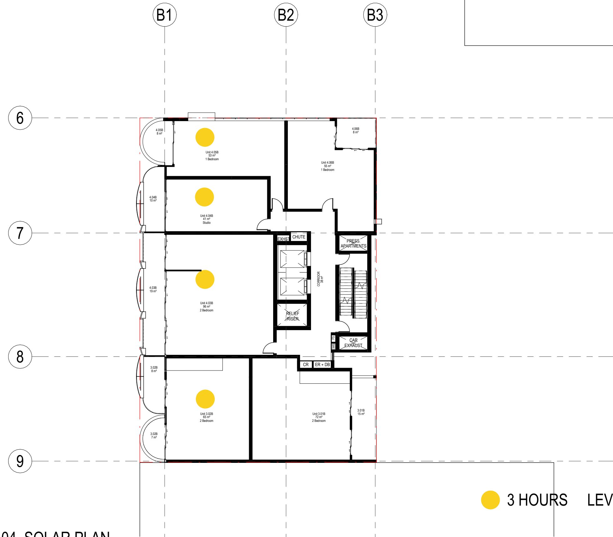
2 LEVEL 04_SOLAR PLAN DA08.01 1 : 200
