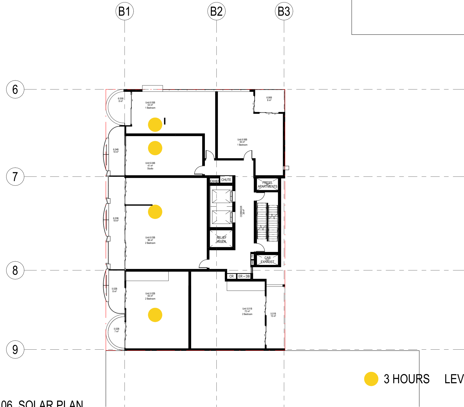
2 LEVEL 06_SOLAR PLAN DA08.01 1:200
