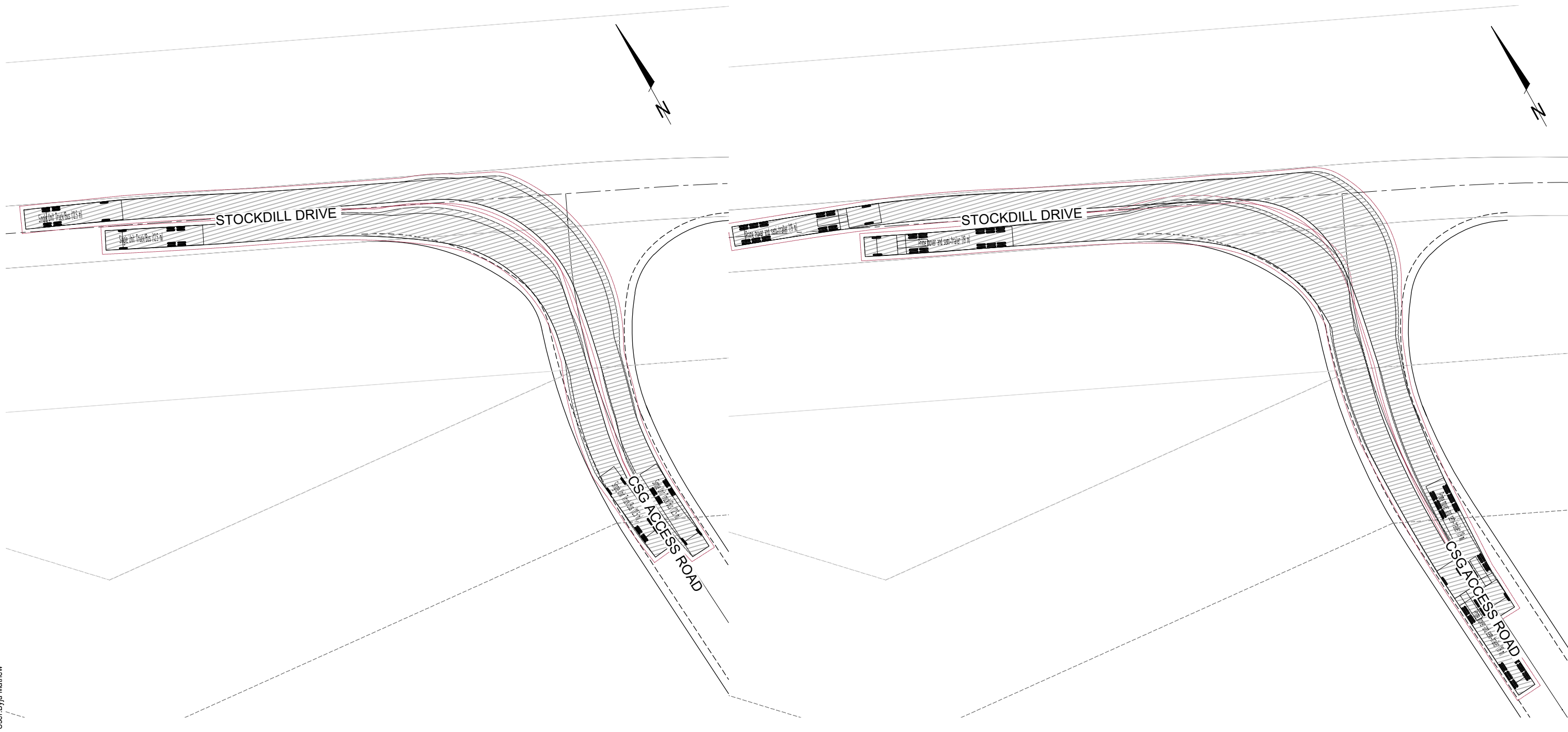
12.5m RIGID TRUCK DESIGN VEHICLE
