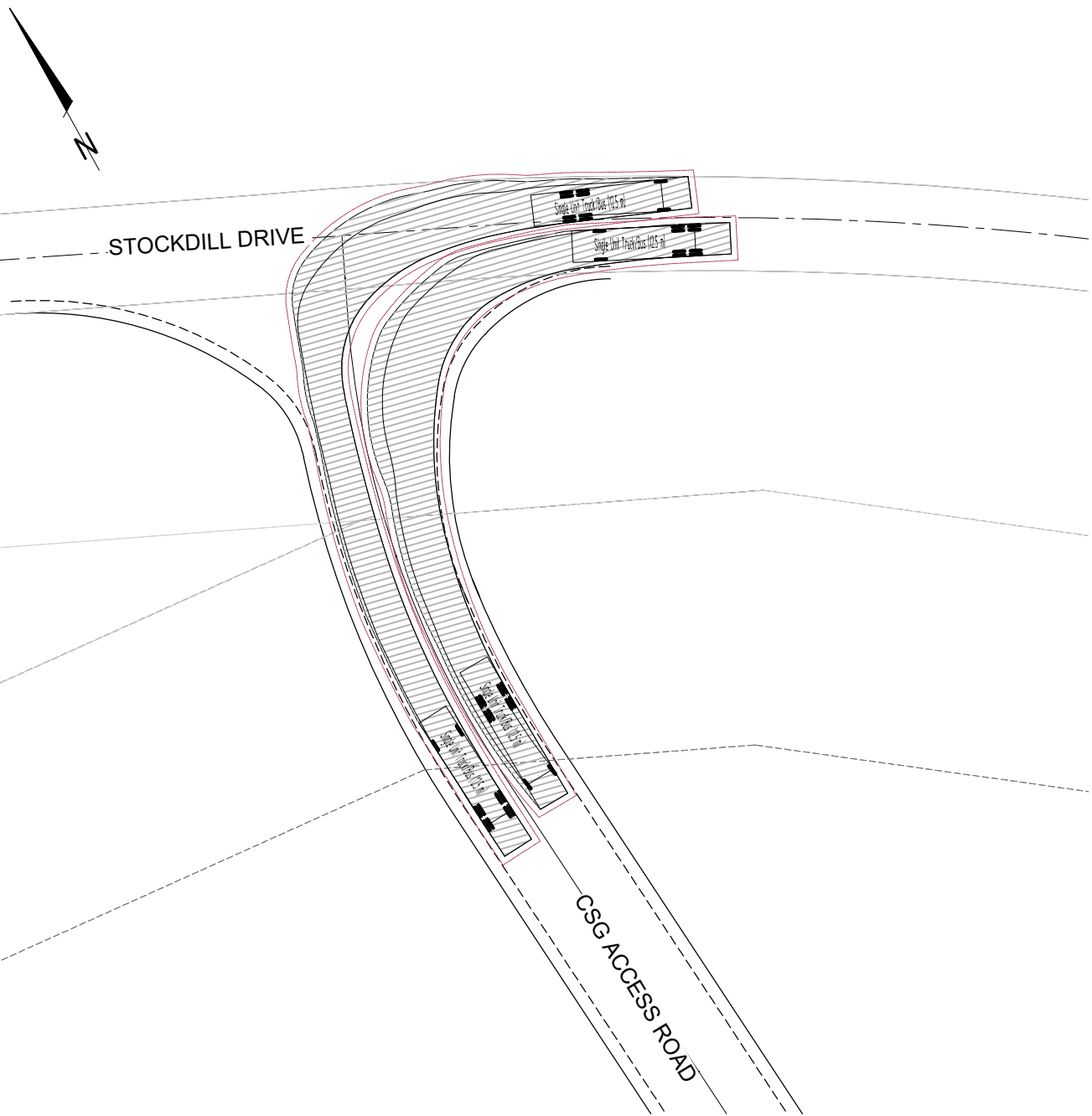
12.5m RIGID TRUCK DESIGN VEHICLE
