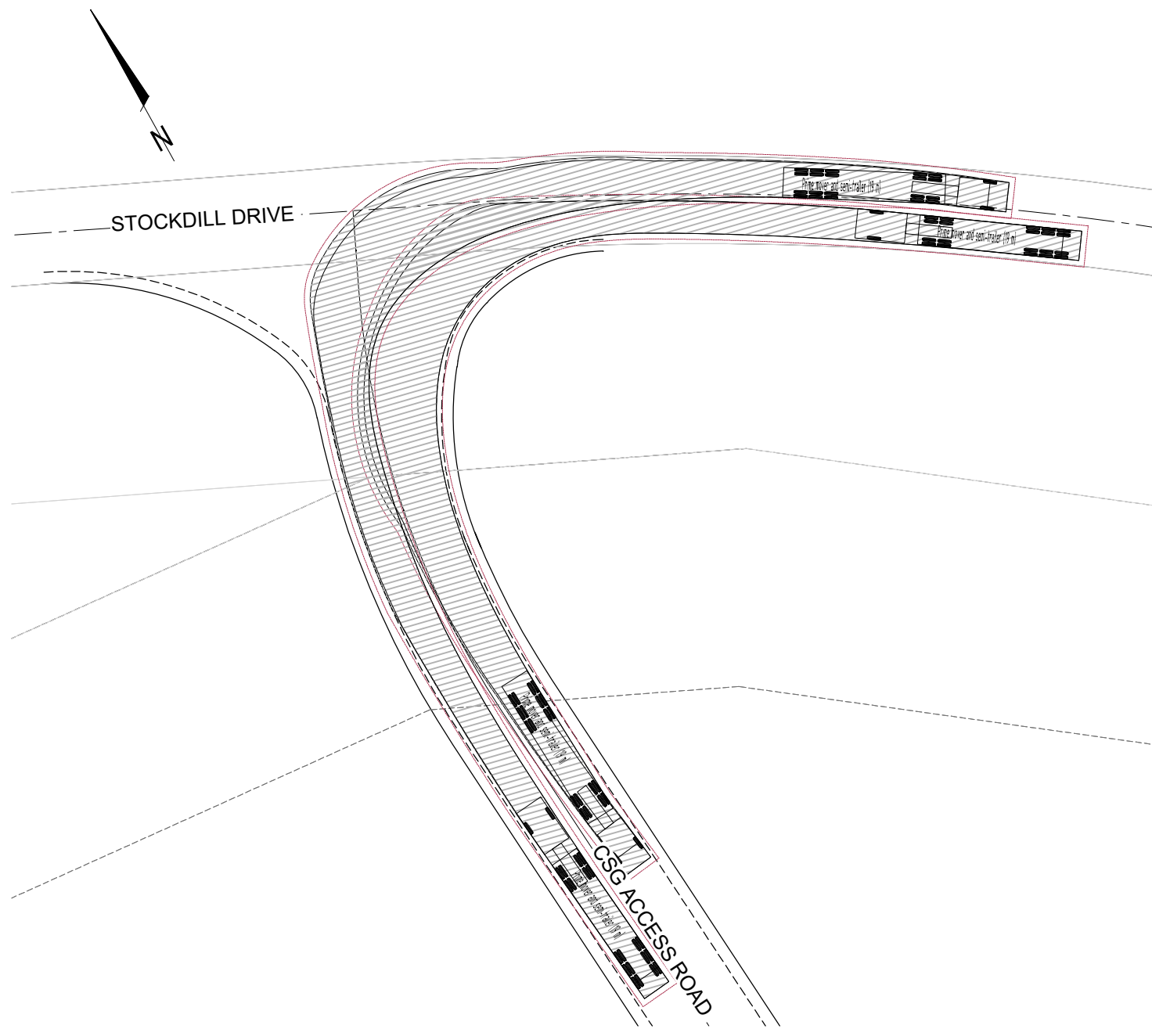
19.0m SEMI TRAILER CHECK VEHICLE
