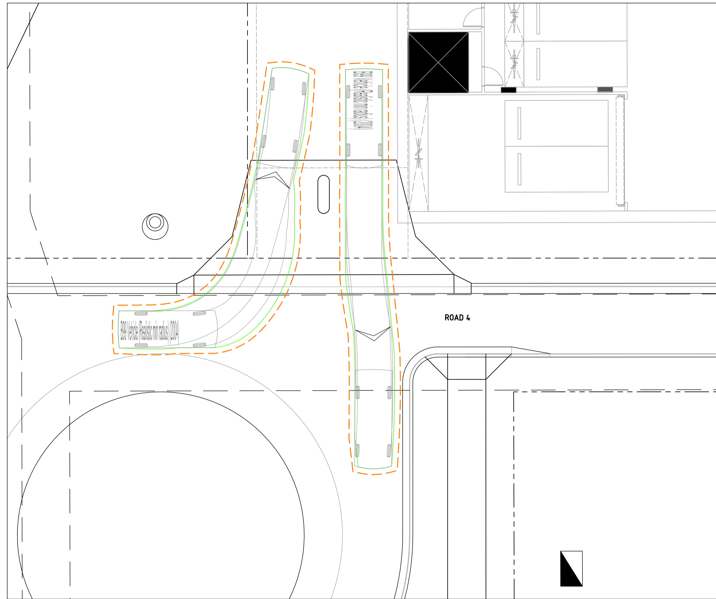
B99 ENTRY/EXIT TO BASEMENT RAMP SCALE 1:100
