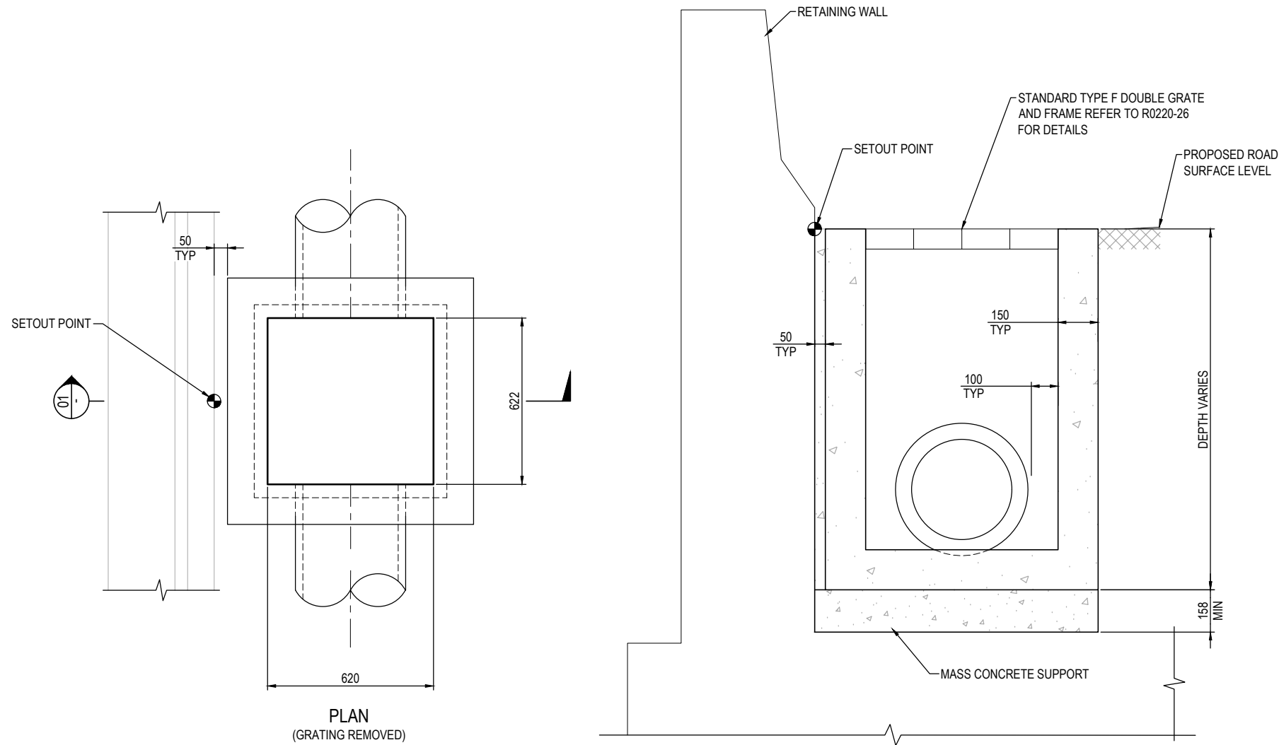
SECTION SCALE 1:10
