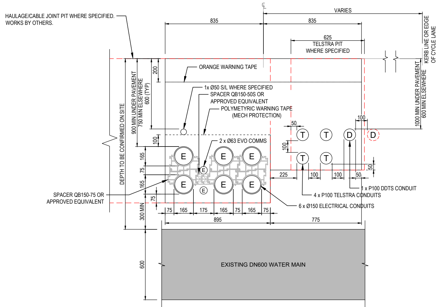
SHARED TRENCH 2 (ST2) CROSSING DN600 WATER MAIN TYPICAL DETAILS 1:10
