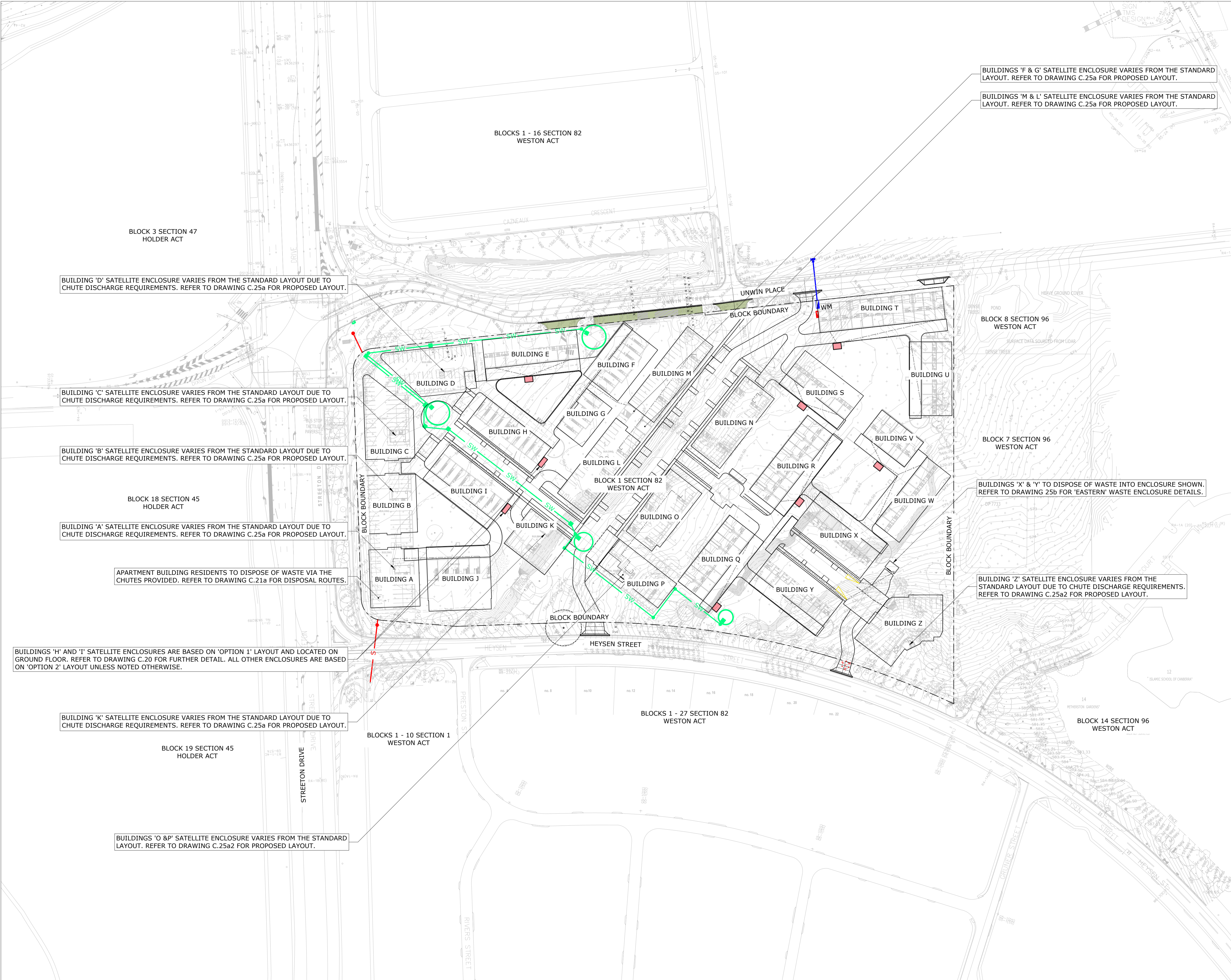
WASTE SCHEMATIC PLAN 1:1000 @ A1
